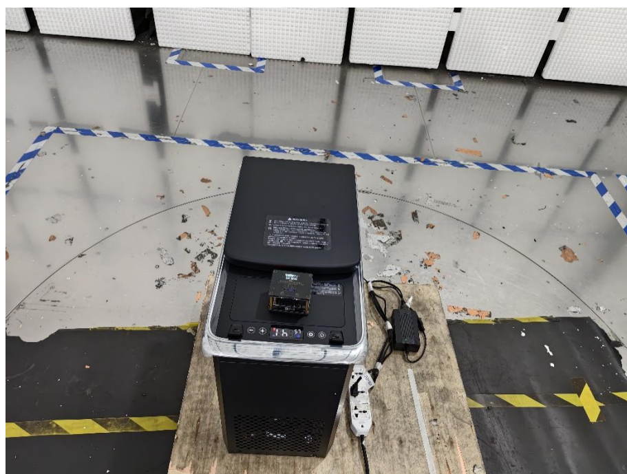
Radiation Emission Test Setup (close up)
