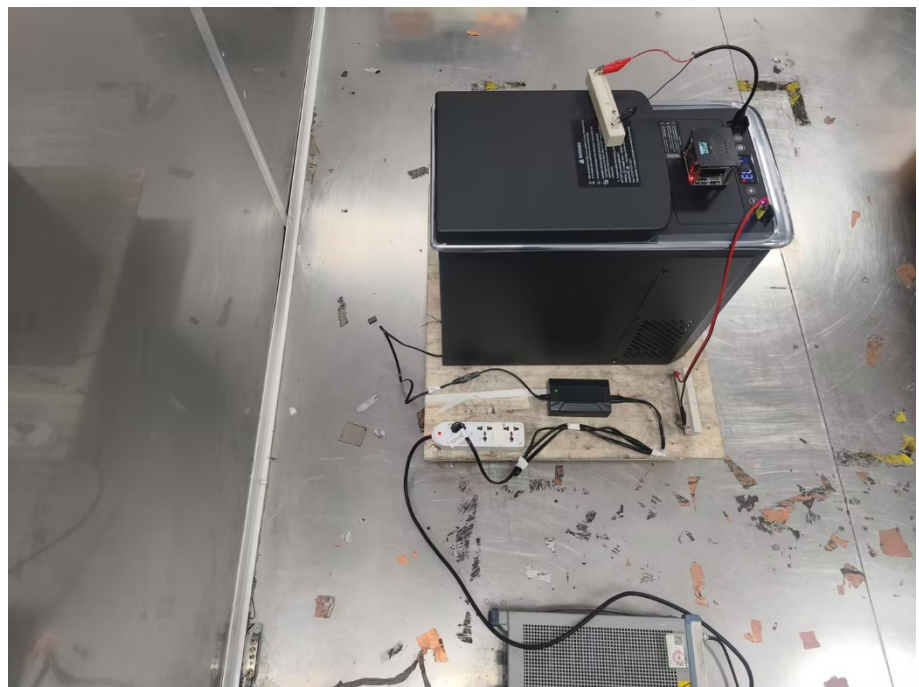
Conducted Emission Test Setup(close up)
