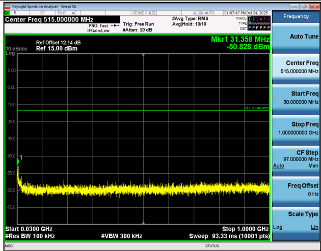
3DH5-Ant1-2441-30~1000-PASS
