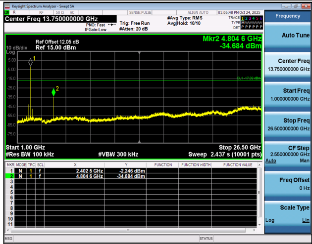
3DH5-Ant1-2402-1000~26500-PASS
