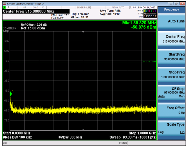
3DH5-Ant1-2402-30~1000-PASS
