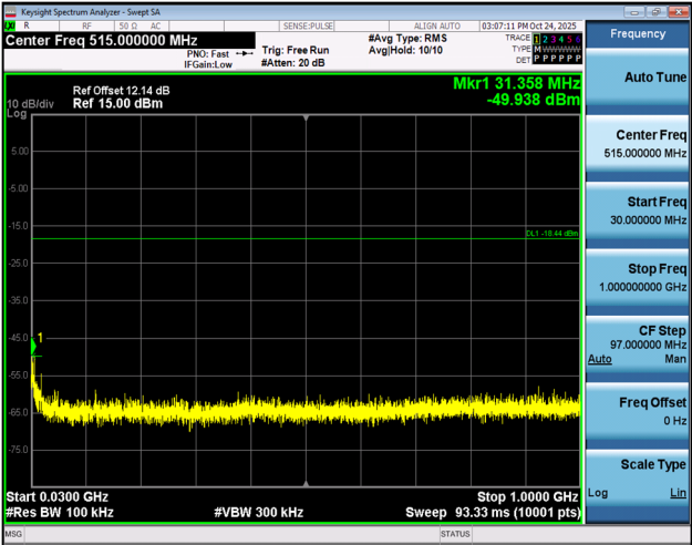
3DH5-Ant1-2441-30~1000-PASS
