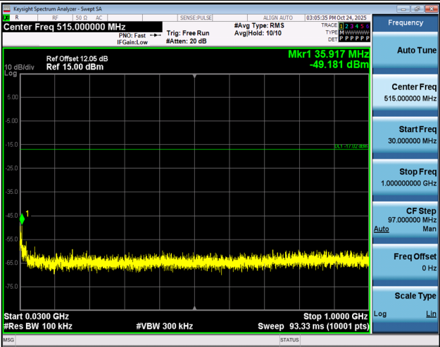
3DH5-Ant1-2402-30~1000-PASS
