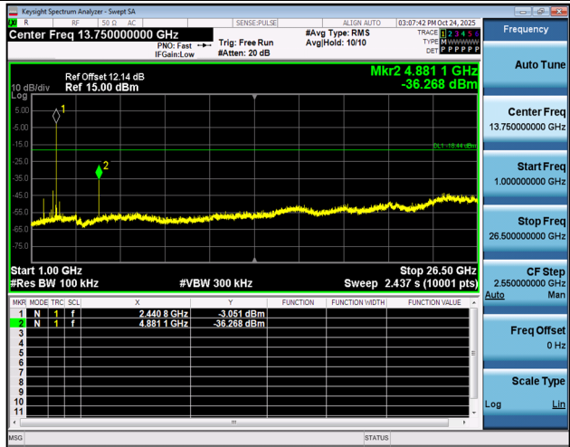
3DH5-Ant1-2441-1000~26500-PASS
