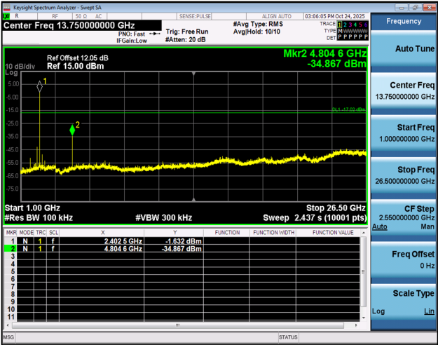
3DH5-Ant1-2402-1000~26500-PASS
