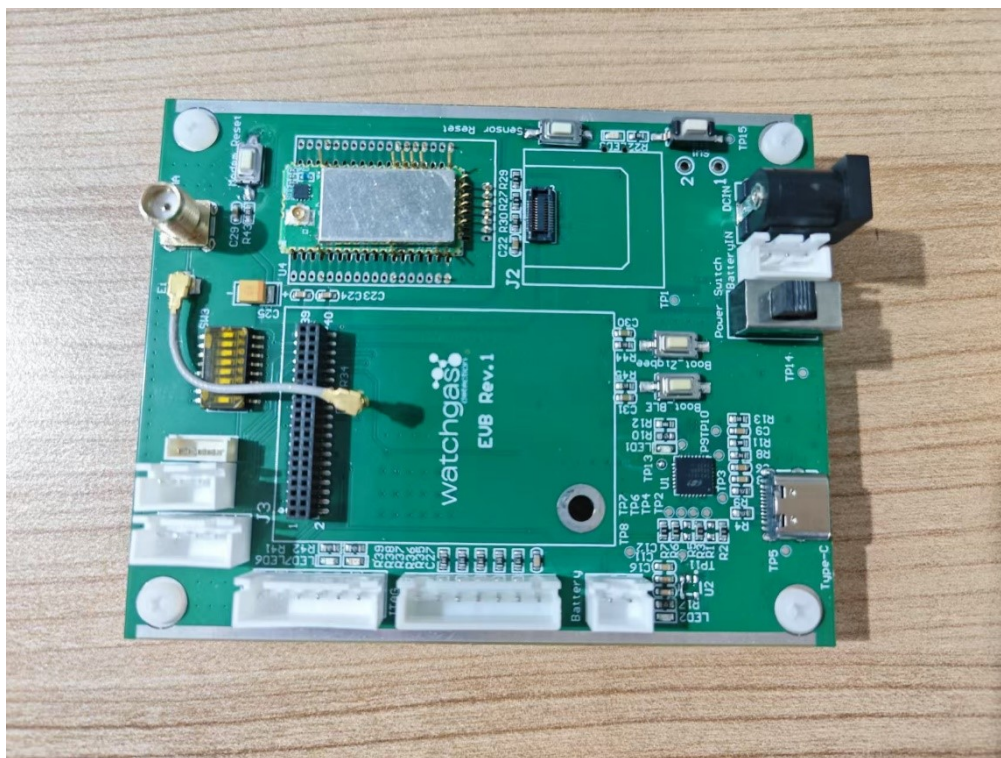
Photograph 2: Set-up photo for RF Conducted Test
