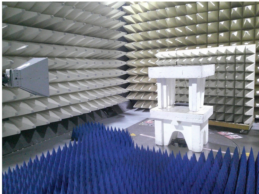
Photograph 4: Set-up photo for Radiated Emission, 1GHz - 10GHz
