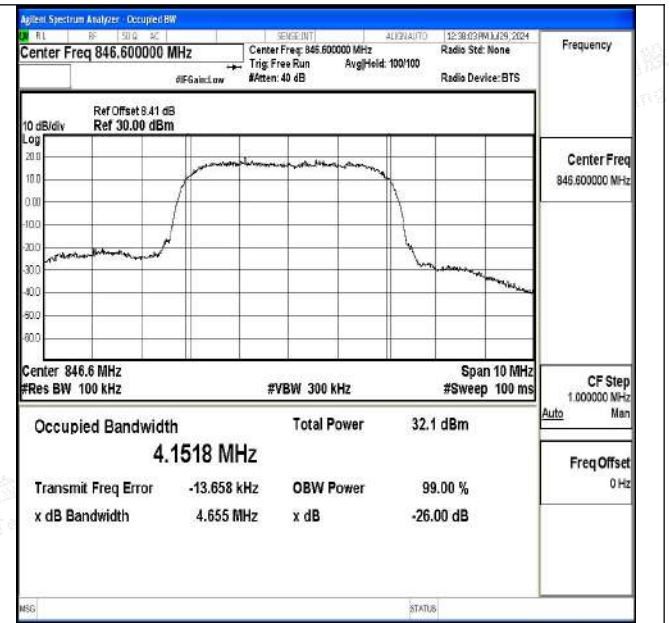
Channel 4233 / 846.6 MHz
