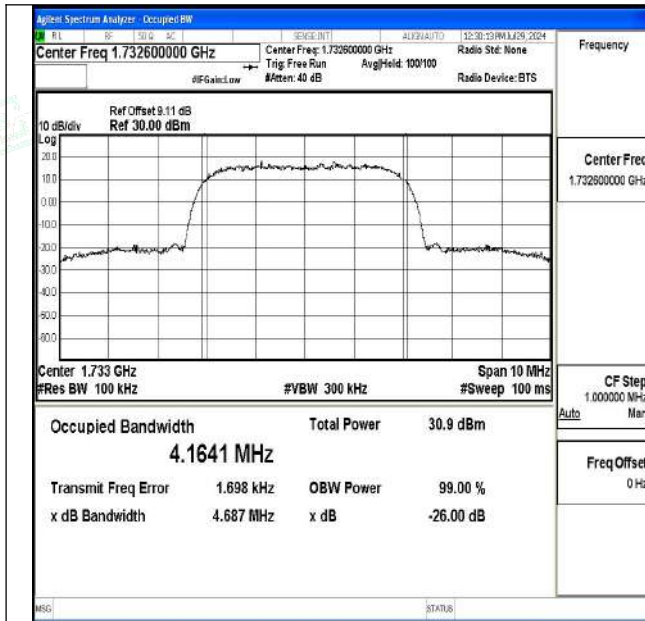
Channel 1413 / 1732.6 MHz
