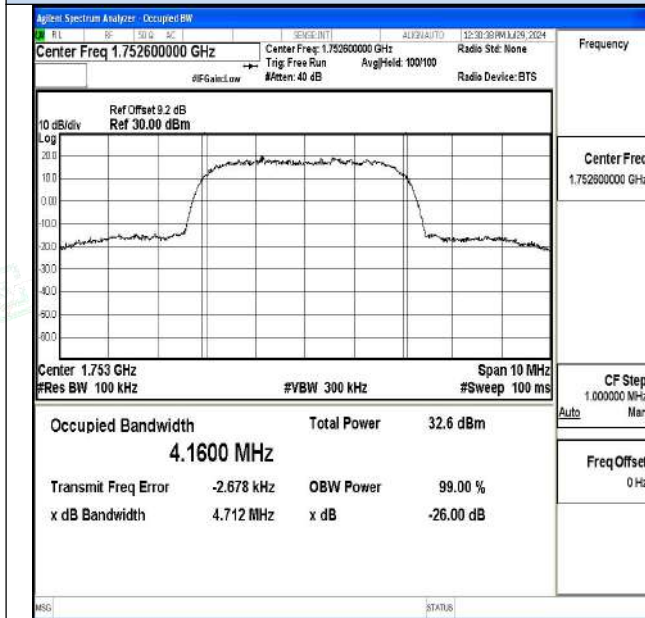
Channel 1513 / 1752.6 MHz
