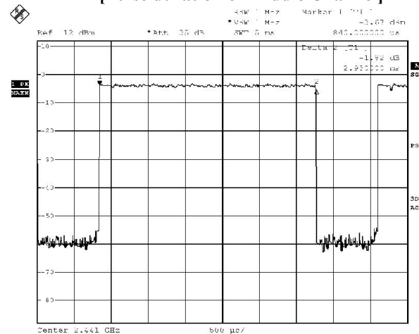
[Pulse duration of Middle Channel]
