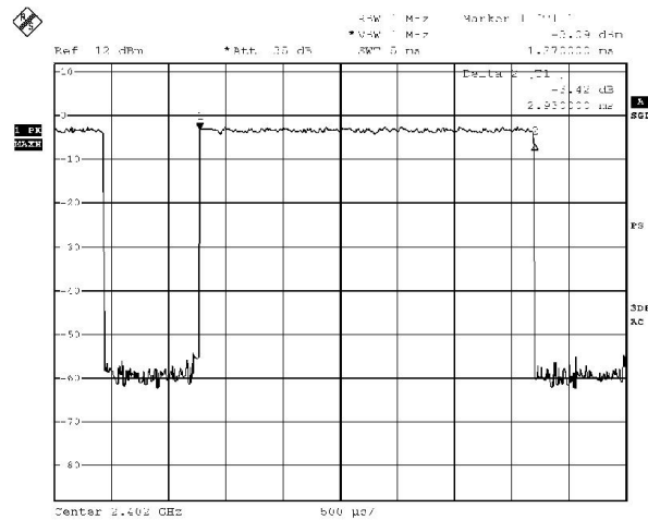
[Pulse duration of Lowest Channel]
