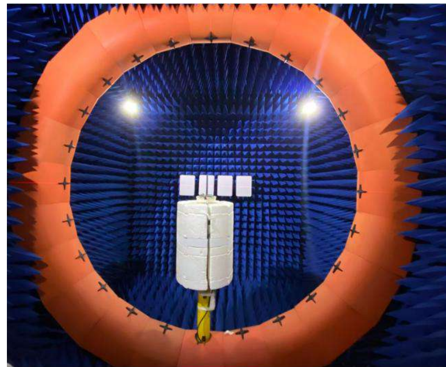
Testing 3D microwave darkroom(3m*3m*3m)
