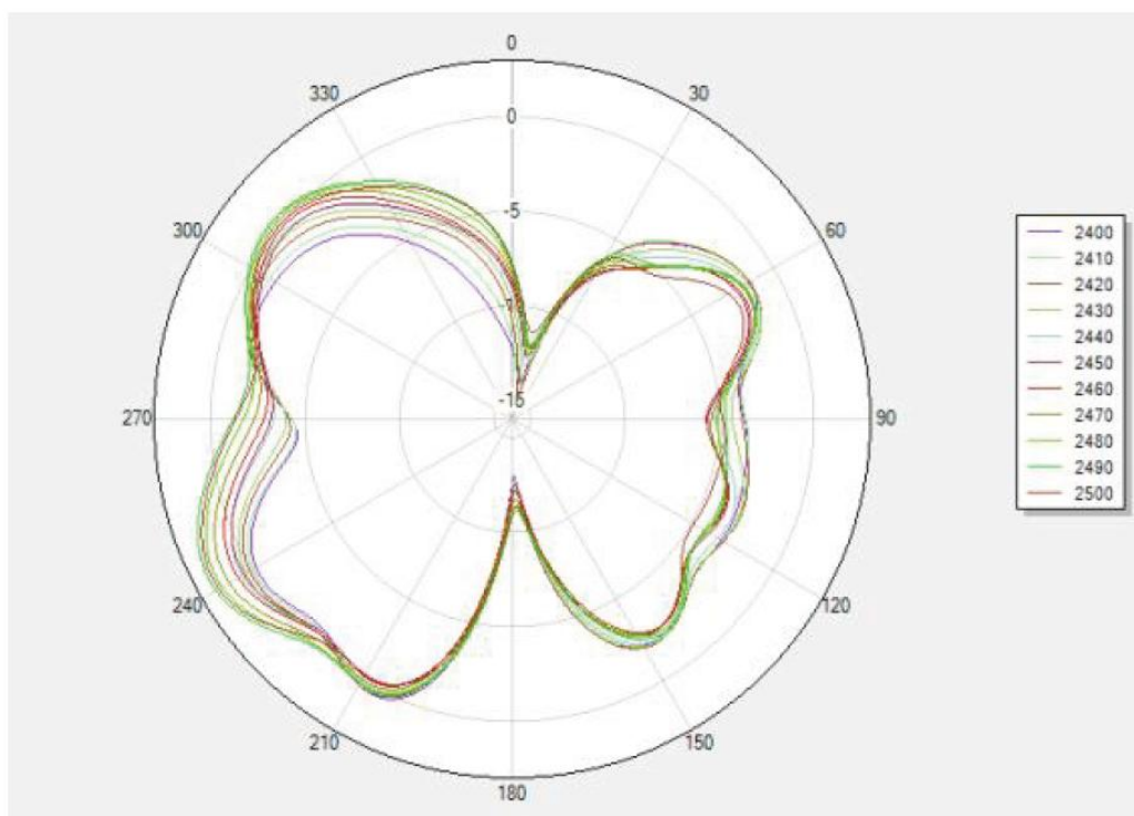
Phi 90 2D
