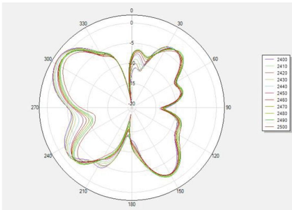
Phi 90 2D
