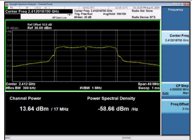
11G-Ant1-2412-PASS
