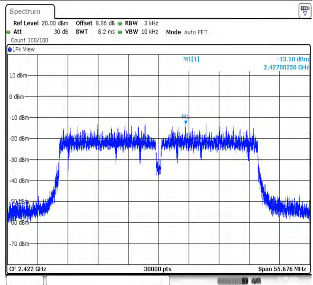
11N40SISO-Ant1-2422-PASS
