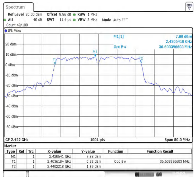
11N40SISO-Ant1-2422
