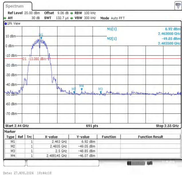
11B-Ant1-2462-PASS
