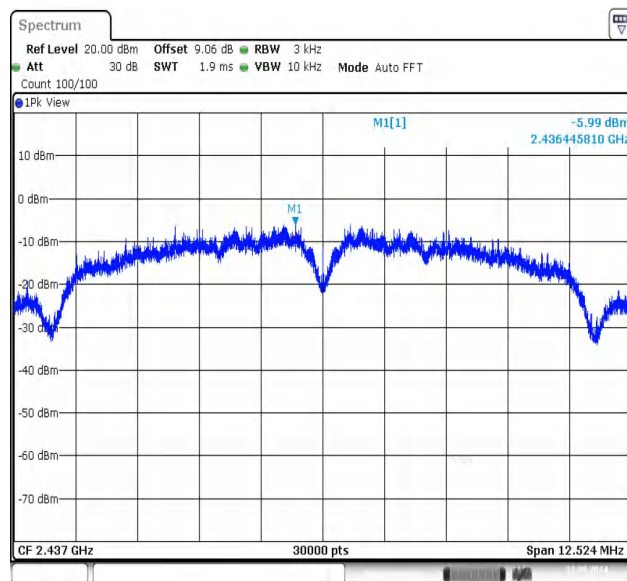
11B-Ant1-2437-PASS
