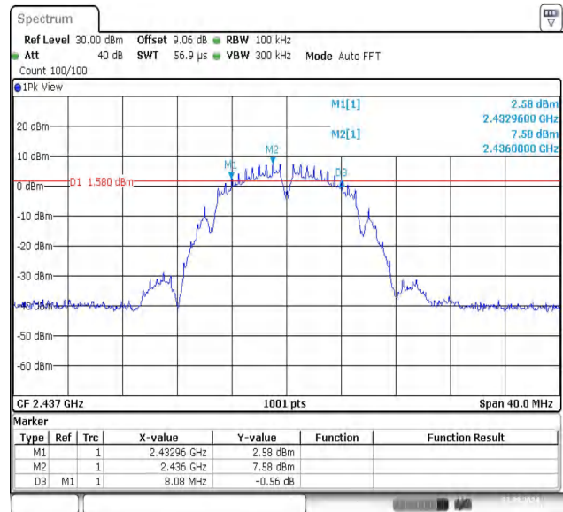
11B-Ant1-2437-PASS
