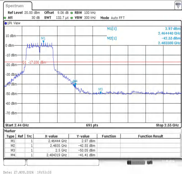
11G-Ant1-2462-PASS
