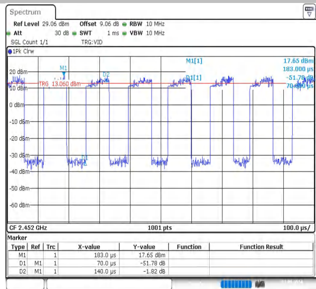
NTNV-11N40SISO-Ant1-2452
