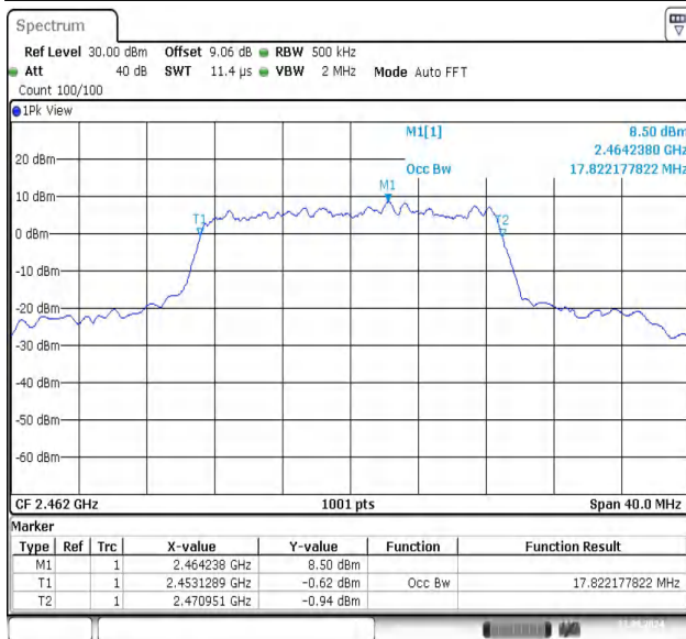
11N20SISO-Ant1-2462
