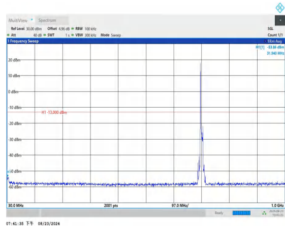
Band17_10MHz_QPSK_23780_1RB#0_30~1000_30~1000
