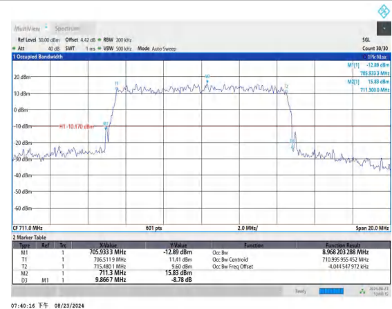
Band17-10MHz-16QAM-23800-50RB#0-PASS
