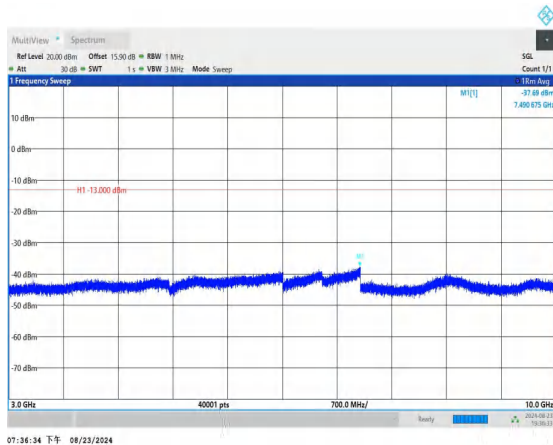
Band17_5MHz_QPSK_23825_1RB#0_3000~10000_3000~1000
