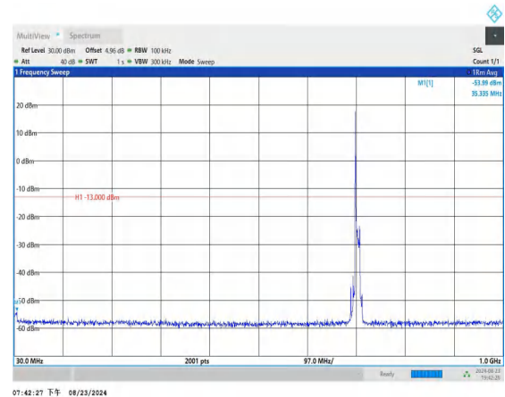
Band17_10MHz_QPSK_23800_1RB#0_30~1000_30~1000
