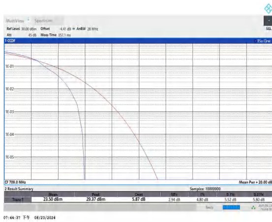
Band17-10MHz-16QAM-23780-1RB#0-PASS
