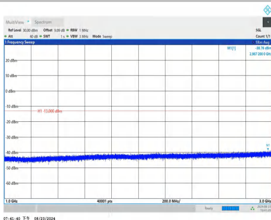
Band17_10MHz_QPSK_23780_1RB#0_1000~3000_1000~3000
