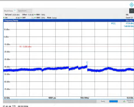
Band17_10MHz_QPSK_23780_1RB#0_3000~10000_3000~1000
