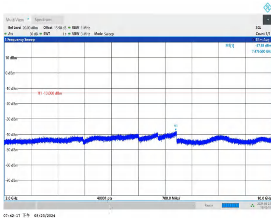
Band17_10MHz_QPSK_23790_1RB#0_3000~10000_3000~10000 00
