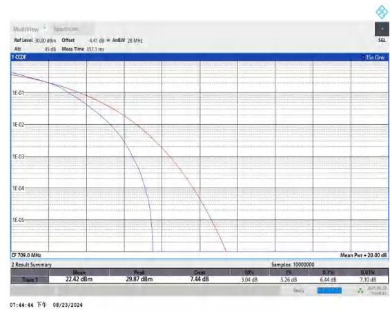
Band17-10MHz-16QAM-23780-50RB#0-PASS
