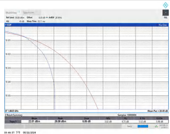
Band25-1.4MHz-16QAM-26365-6RB#0-PASS
