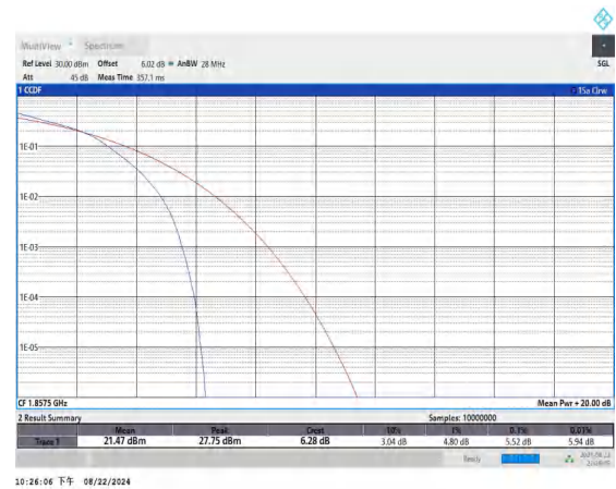
Band25-15MHz-16QAM-26115-75RB#0-PASS
