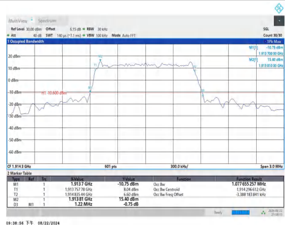
Band25-1.4MHz-16QAM-26683-6RB#0-PASS
