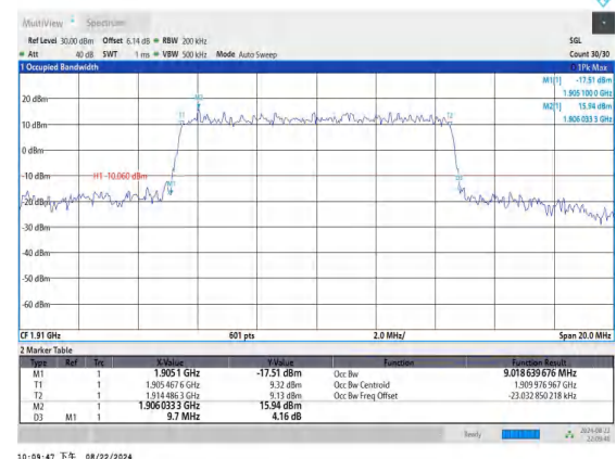
Band25-10MHz-16QAM-26640-50RB#0-PASS
