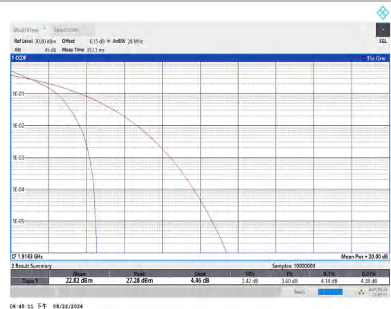
Band25-1.4MHz-QPSK-26683-6RB#0-PASS
