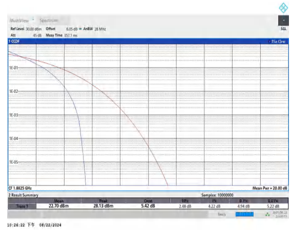
Band25-15MHz-QPSK-26365-75RB#0-PASS
