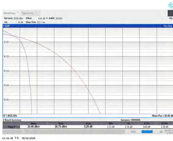
Band25-5MHz-QPSK-26065-1RB#0-PASS
