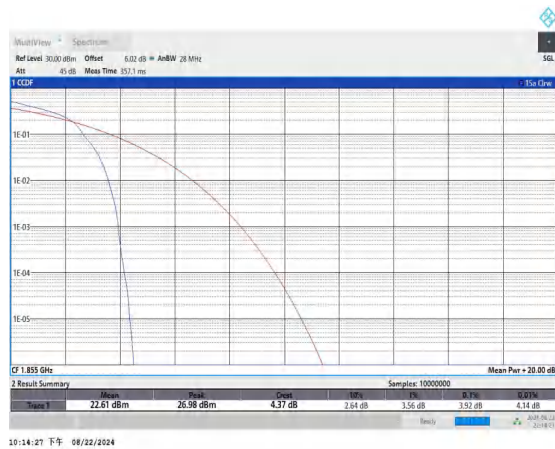
Band25-10MHz-16QAM-26090-1RB#0-PASS
