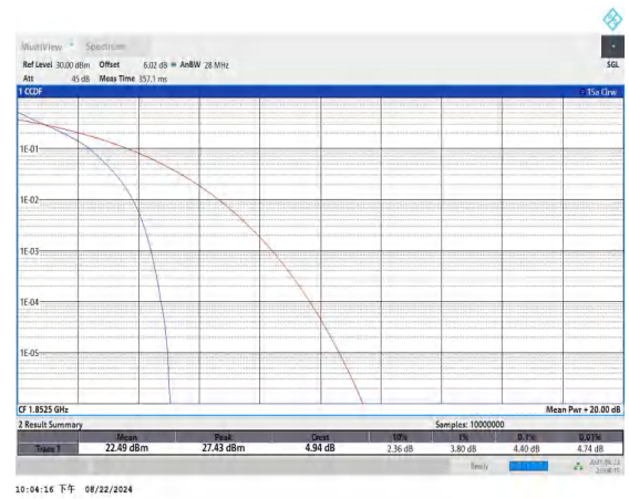
Band25-5MHz-QPSK-26065-25RB#0-PASS
