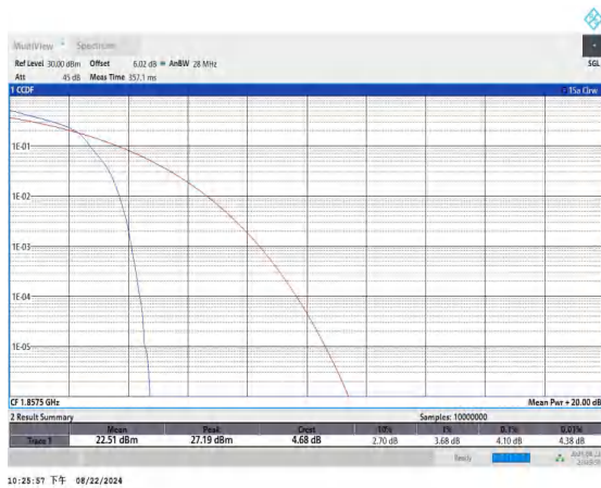
Band25-15MHz-16QAM-26115-1RB#0-PASS
