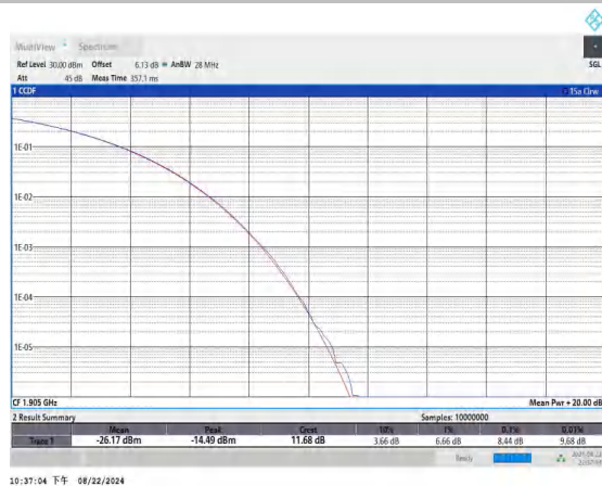
Band25-20MHz-16QAM-26590-1RB#0-PASS
