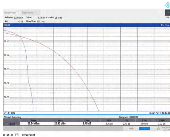
Band25-10MHz-16QAM-26640-1RB#0-PASS
