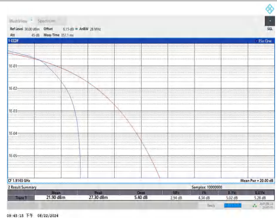
Band25-1.4MHz-16QAM-26683-6RB#0-PASS
