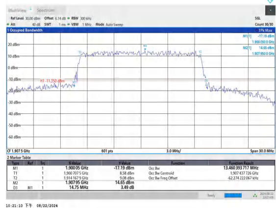
Band25-15MHz-16QAM-26615-75RB#0-PASS
