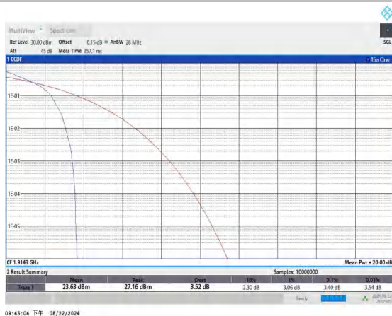
Band25-1.4MHz-QPSK-26683-1RB#0-PASS
