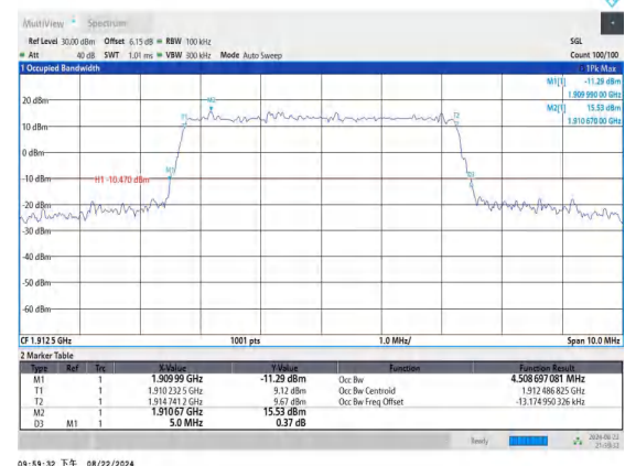
Band25-5MHz-16QAM-26665-25RB#0-PASS
