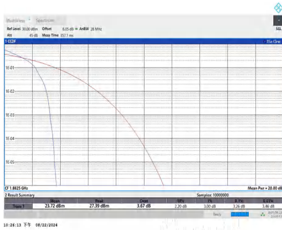
Band25-15MHz-QPSK-26365-1RB#0-PASS
