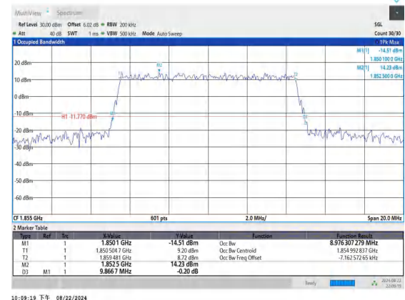
Band25-10MHz-16QAM-26090-50RB#0-PASS
