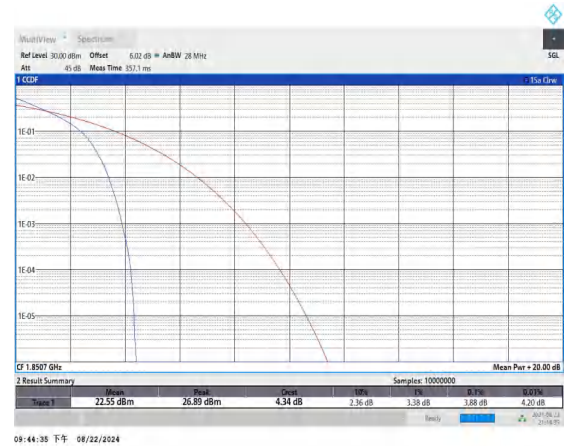
Band25-1.4MHz-QPSK-26047-6RB#0-PASS
