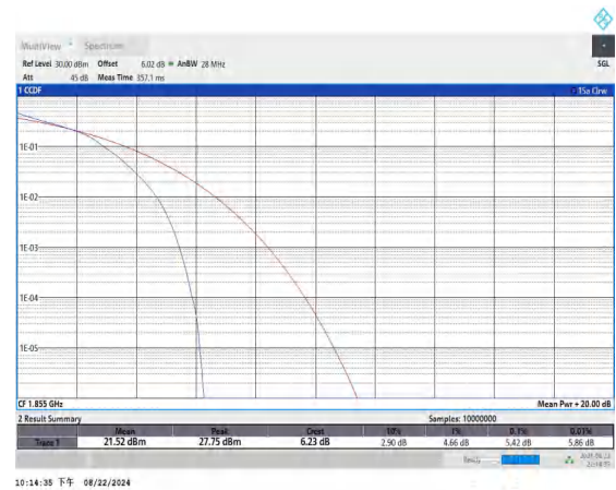
Band25-10MHz-16QAM-26090-50RB#0-PASS
