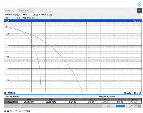
Band25-1.4MHz-16QAM-26047-6RB#0-PASS
