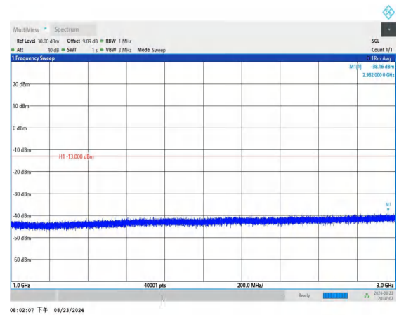
Band26_5MHz_QPSK_26715_1RB#0_1000~3000_1000~3000
