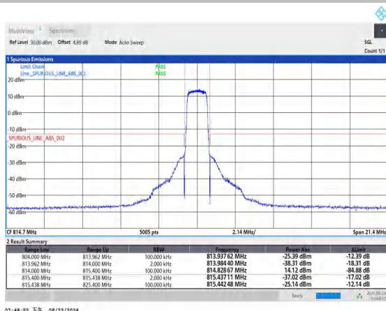
Band26_1.4MHz_QPSK_26697_6RB#0
