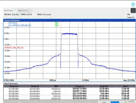
Band26_3MHz_QPSK_26775_1RB#0
