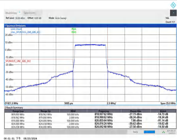
Band26_5MHz_QPSK_26765_25RB#0
