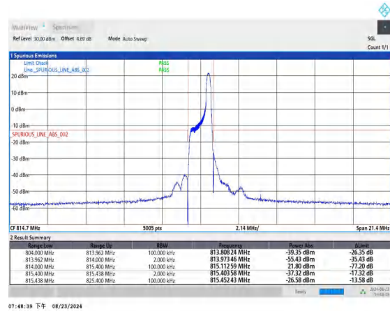
Band26_1.4MHz_QPSK_26697_1RB#5
