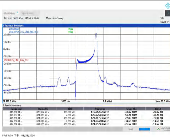
Band26_3MHz_QPSK_26775_1RB#14
