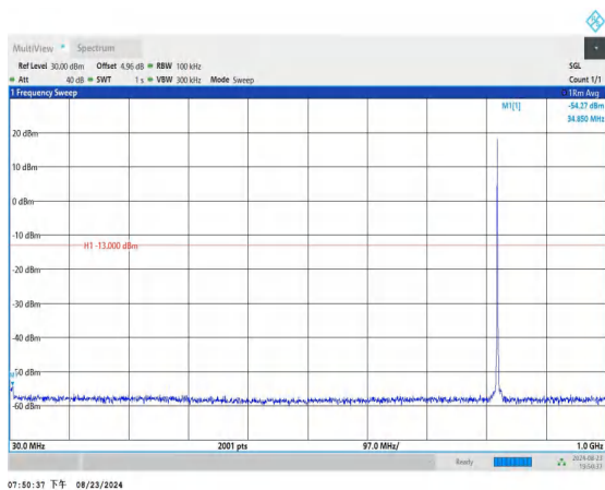
Band26_1.4MHz_QPSK_26783_1RB#0_30~1000_30~1000
