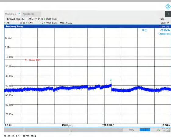
Band26_1.4MHz_QPSK_26740_1RB#0_3000~10000_3000~10 000
