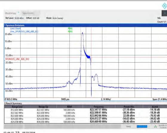
Band26_1.4MHz_QPSK_26783_1RB#0
