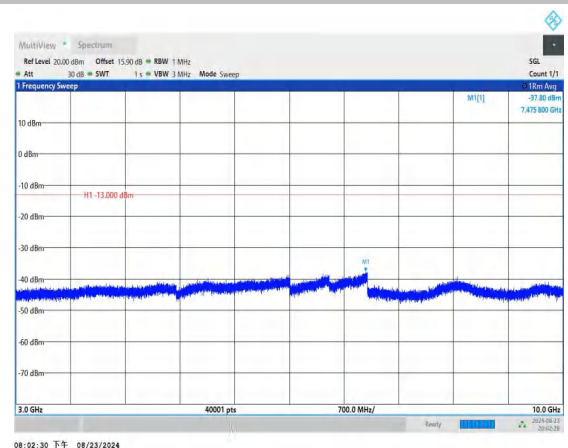
Band26_5MHz_QPSK_26740_1RB#0_3000~10000_3000~1000
