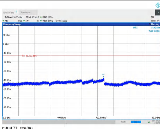
Band26_1.4MHz_QPSK_26697_1RB#0_3000~10000_3000~10 000
