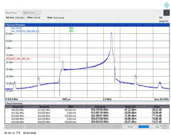
Band26_10MHz_QPSK_26740_1RB#49
