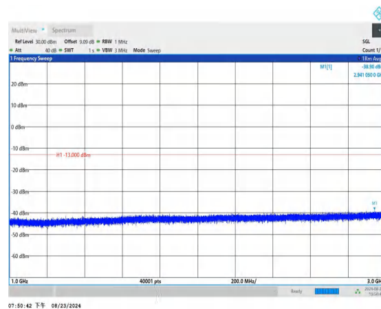
Band26_1.4MHz_QPSK_26783_1RB#0_1000~3000_1000~3000
