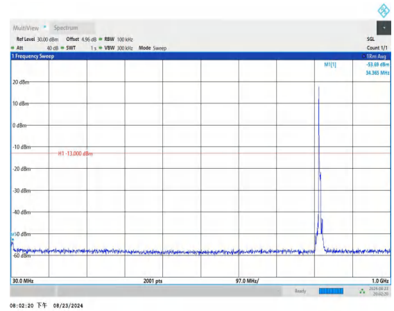
Band26_5MHz_QPSK_26740_1RB#0_30~1000_30~1000
