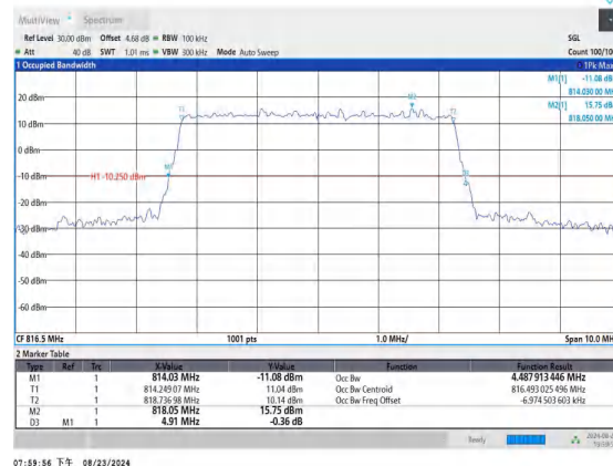
26(814-824)-5MHz-16QAM-26715-25RB#0-PASS
