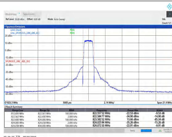
Band26_1.4MHz_QPSK_26783_6RB#0
