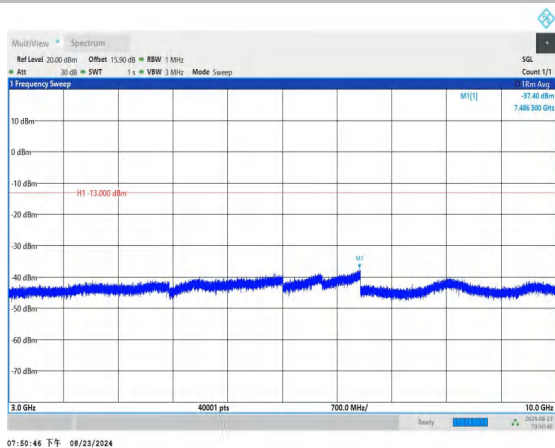
Band26_1.4MHz_QPSK_26783_1RB#0_3000~10000_3000~10000
