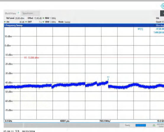
Band26_3MHz_QPSK_26705_1RB#0_3000~10000_3000~10000
