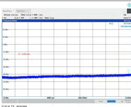
Band26_1.4MHz_QPSK_26740_1RB#0_1000~3000_1000~300 0
