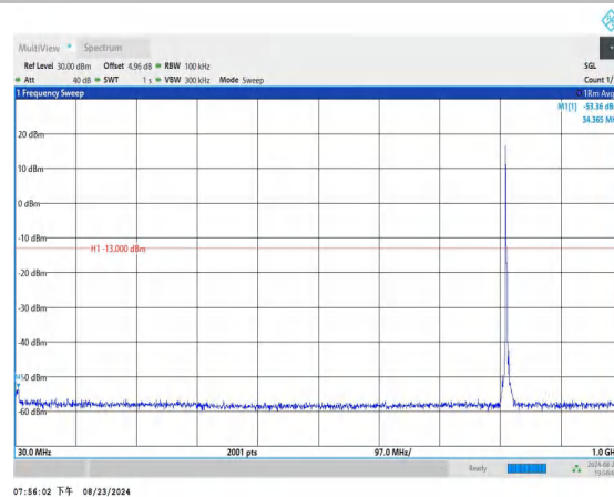
Band26_3MHz_QPSK_26705_1RB#0_30~1000_30~1000
