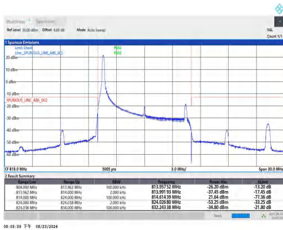
Band26_10MHz_QPSK_26740_1RB#0
