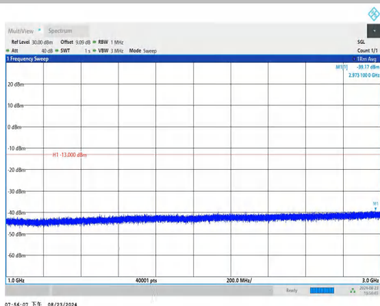
Band26_3MHz_QPSK_26705_1RB#0_1000~3000_1000~3000
