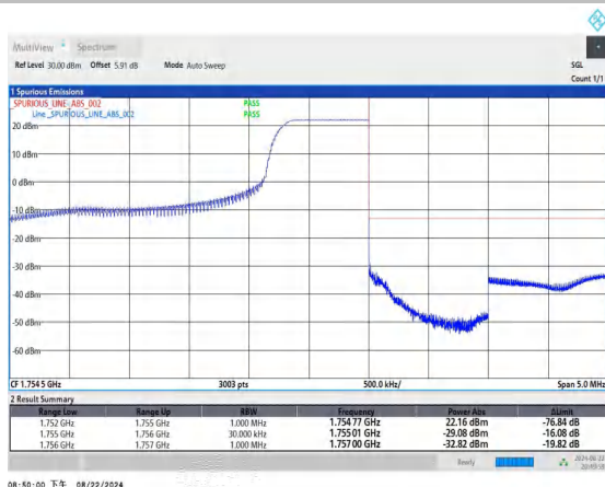
Band4_3MHz_QPSK_20385_1RB#14
