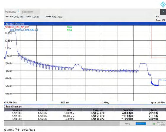
Band4_20MHz_16QAM_20300_1RB#0
