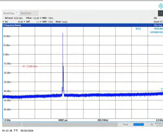
Band4_10MHz_QPSK_20350_1RB#0_1000~3000_1000~3000
