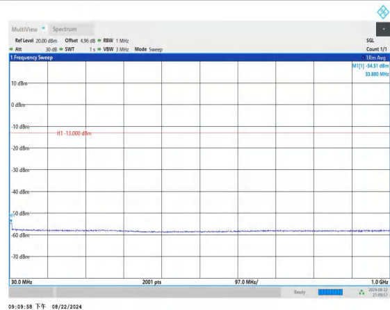
Band4_10MHz_QPSK_20000_1RB#0_30~1000_30~1000
