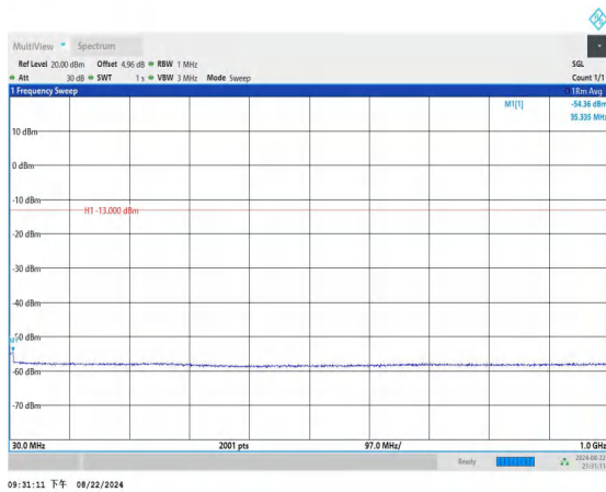
Band4_20MHz_QPSK_20175_1RB#0_30~1000_30~1000
