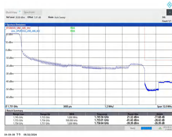
Band4_10MHz_16QAM_20350_1RB#0
