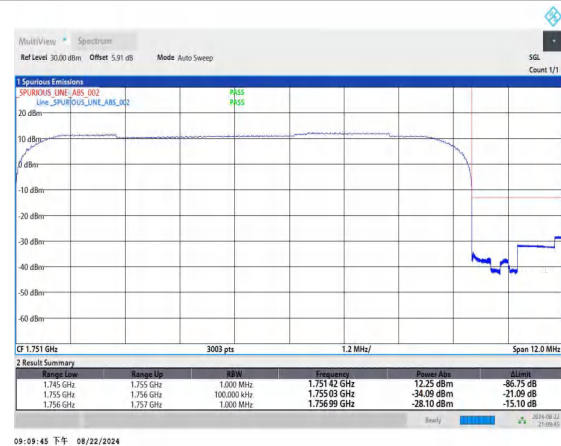
Band4_10MHz_16QAM_20350_50RB#0
