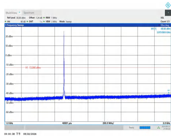
Band4_5MHz_QPSK_19975_1RB#0_1000~3000_1000~3000
