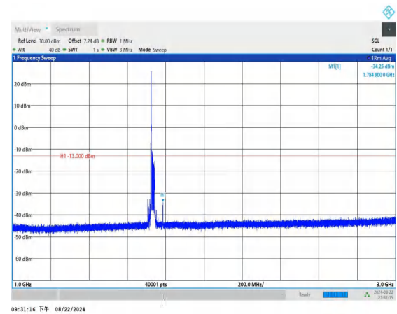
Band4_20MHz_QPSK_20175_1RB#0_1000~3000_1000~3000
