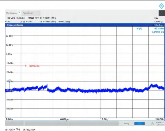
Band4_20MHz_QPSK_20300_1RB#0_3000~20000_3000~2000
