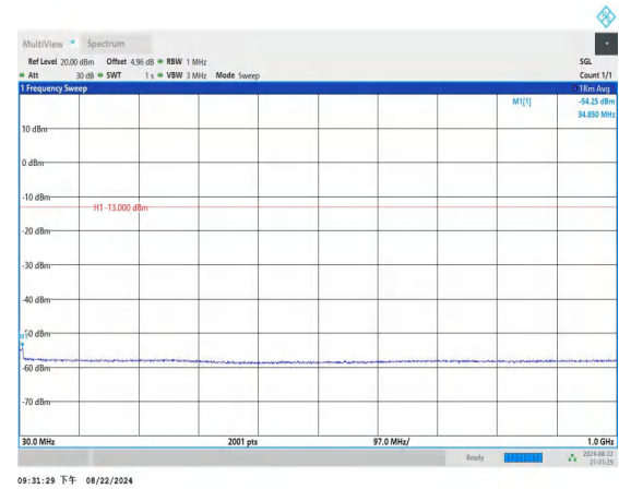
Band4_20MHz_QPSK_20300_1RB#0_30~1000_30~1000
