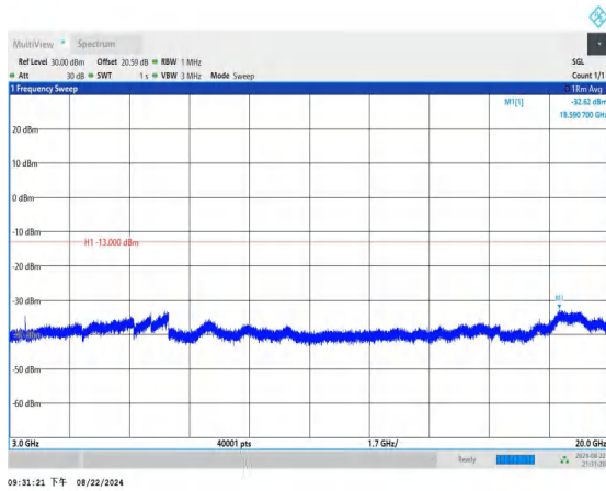
Band4_20MHz_QPSK_20175_1RB#0_3000~20000_3000~2000
