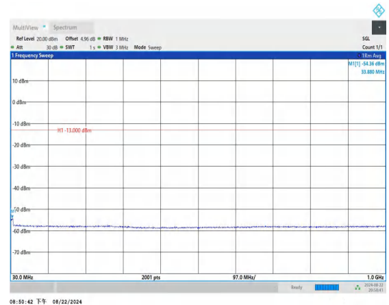
Band4_3MHz_QPSK_19965_1RB#0_30~1000_30~1000
