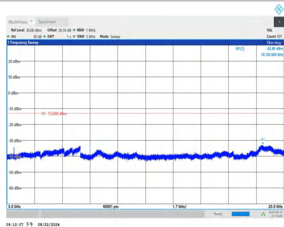
Band4_10MHz_QPSK_20000_1RB#0_3000~20000_3000~20000
