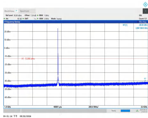
Band4_5MHz_QPSK_20375_1RB#0_1000~3000_1000~3000
