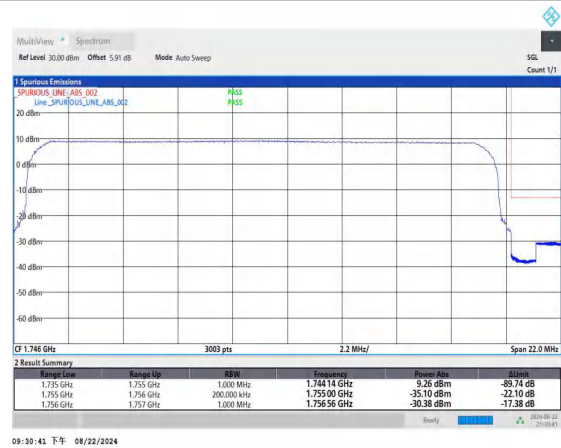
Band4_20MHz_16QAM_20300_100RB#0
