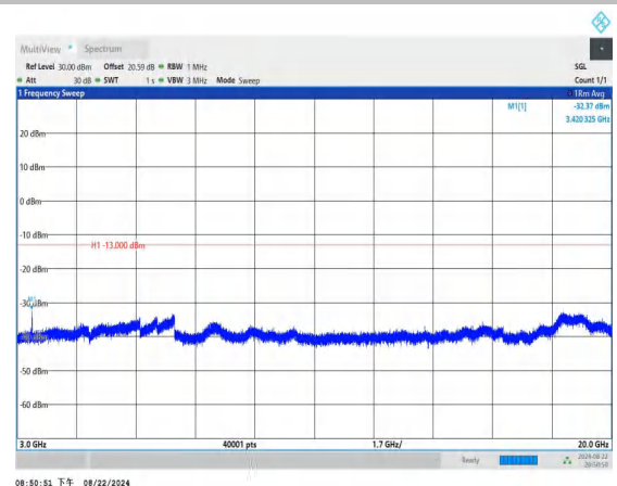
Band4_3MHz_QPSK_19965_1RB#0_3000~20000_3000~20000
