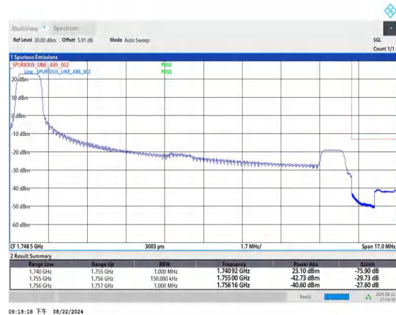
Band4_15MHz_QPSK_20325_1RB#74
