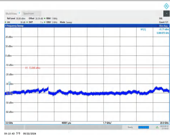
Band4_10MHz_QPSK_20350_1RB#0_3000~20000_3000~2000
