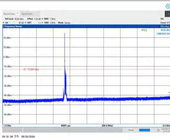
Band4_20MHz_QPSK_20300_1RB#0_1000~3000_1000~3000
