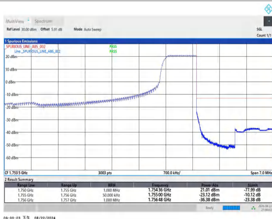
Band4_5MHz_16QAM_20375_1RB#24
