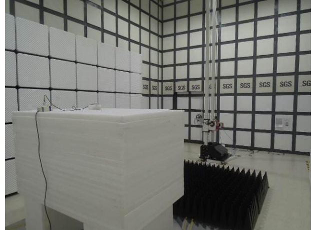
FCC_15_247_BLE_Radiated_Setup
