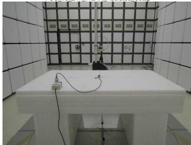
FCC_15_407_WLAN_Radiated_Setup
