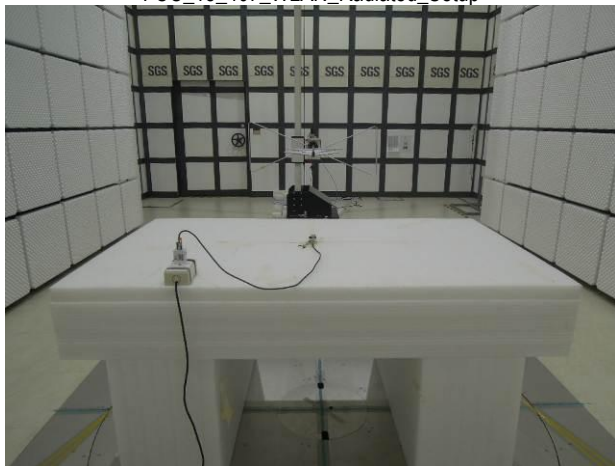
FCC_15_407_WLAN_Radiated_Setup
