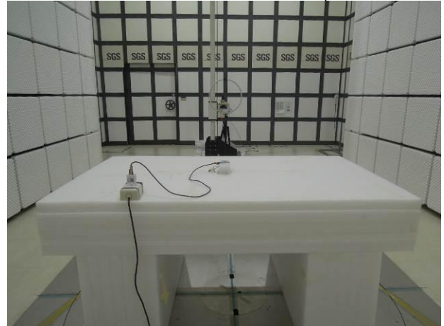
FCC_15_247_BT_Radiated_Setup
