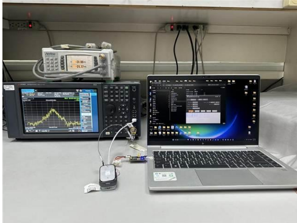
FCC_15_247_WLAN_Conducted_Setup
