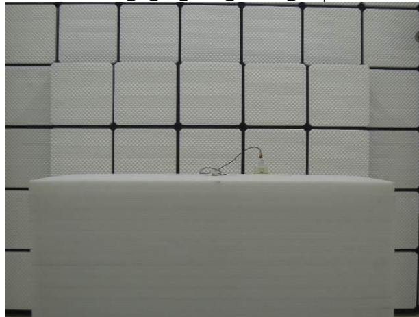
FCC_15_407_WLAN_Radiated_Setup
