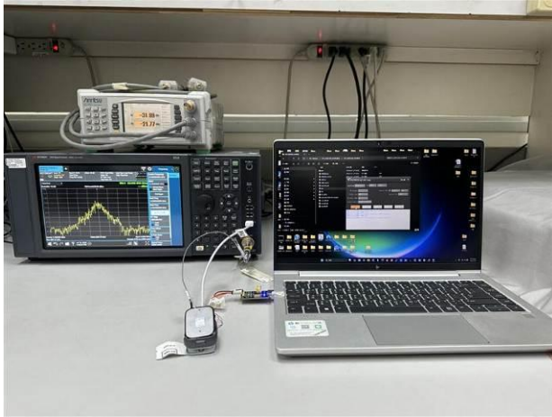
FCC_15_247_BT_Conducted_Setup
