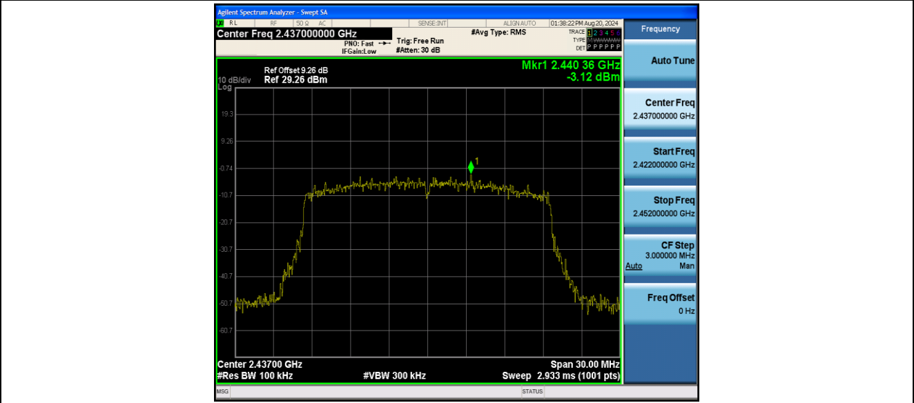
11AX20SISO_Ant1_2437_0-Reference
