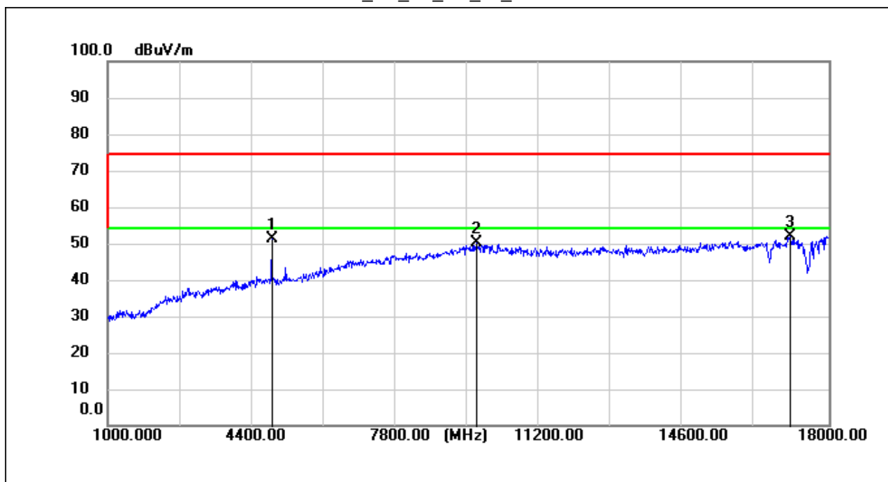
BLE_2M_TX_CH_19_Verical
