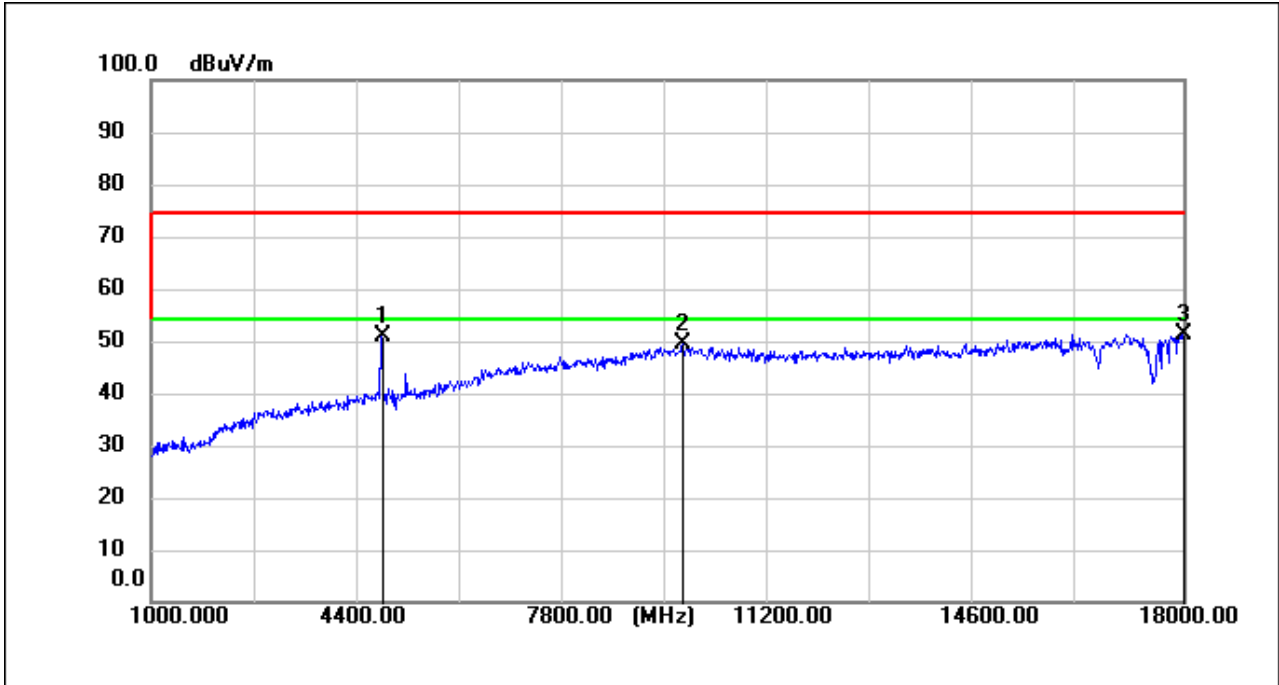
BLE_1M_TX_CH_00_Verical
