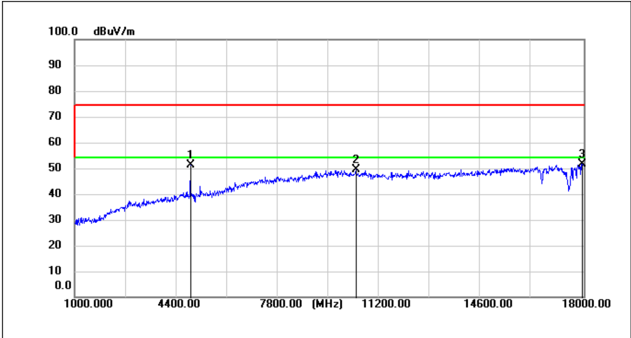
BLE_1M_TX_CH_19_Verical
