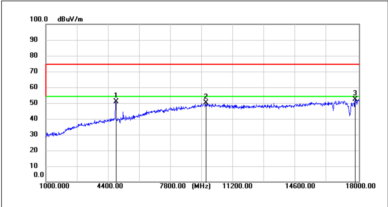
BLE_2M_TX_CH_00_Verical
