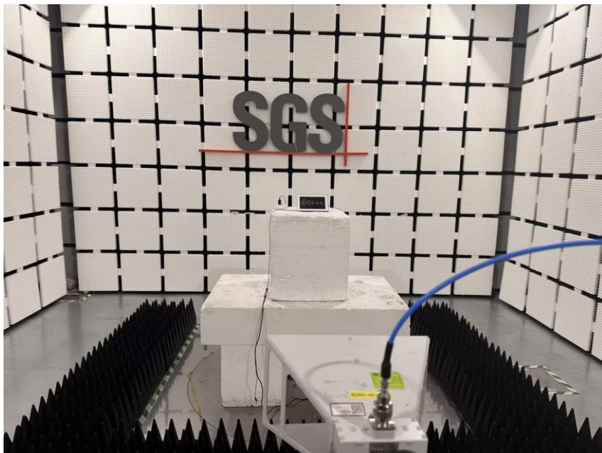
RF Radiated Test Above 1GHz for WiFi
