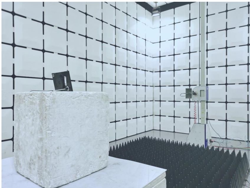
RF Radiated Test (1-18GHz) for 24GHz
