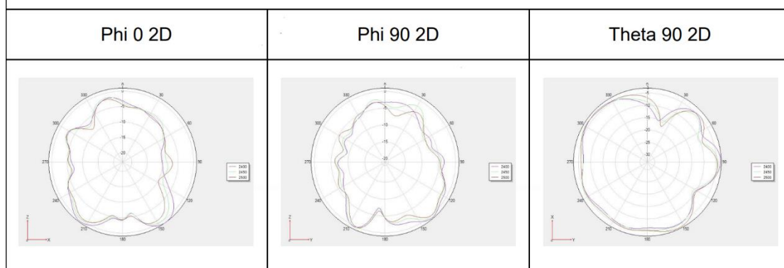
2D-Etotal (2400/2450/2500Mhz)
