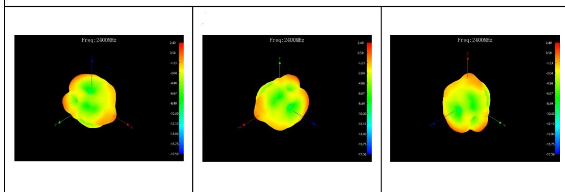
3D-Etotal (2400Mhz)
