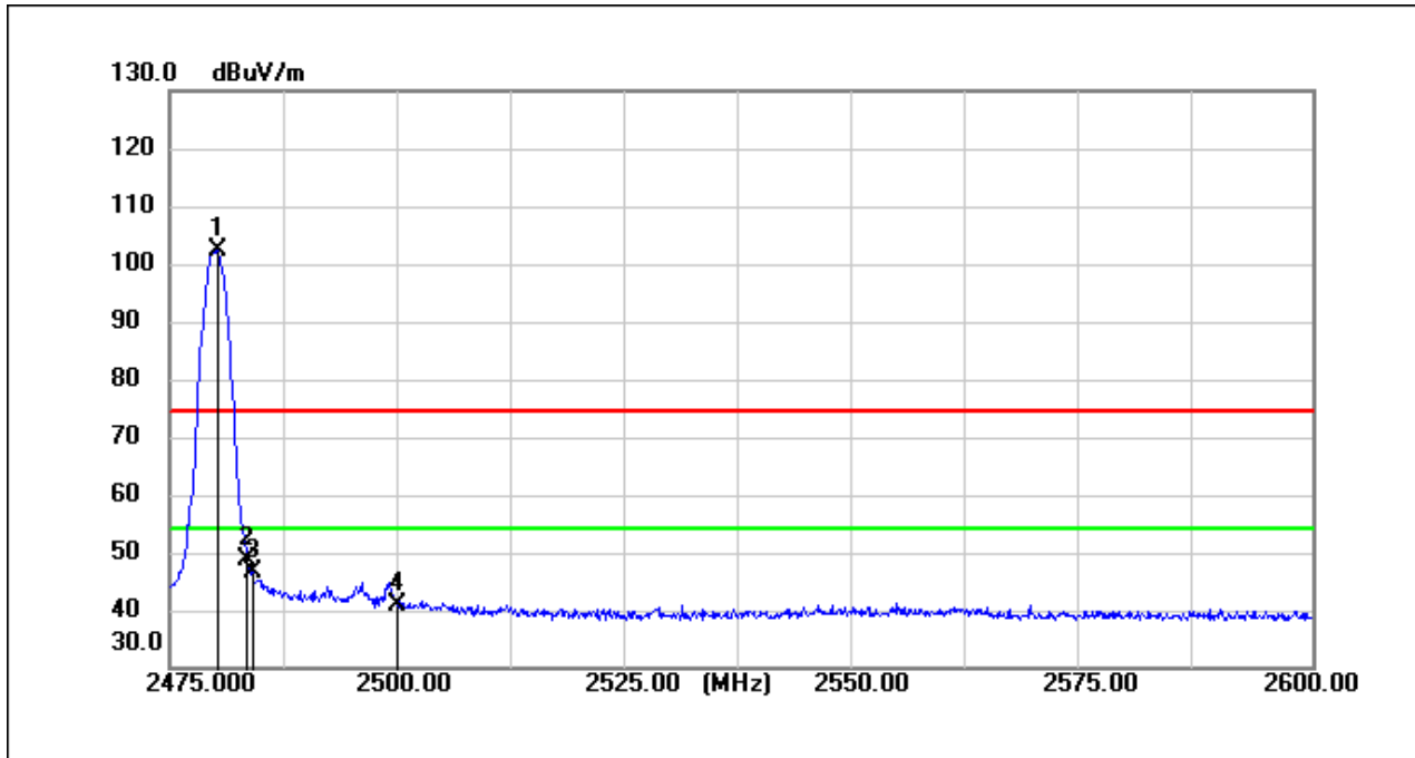
BT_2DH5_TX_CH_78_Horizontal_Peak
