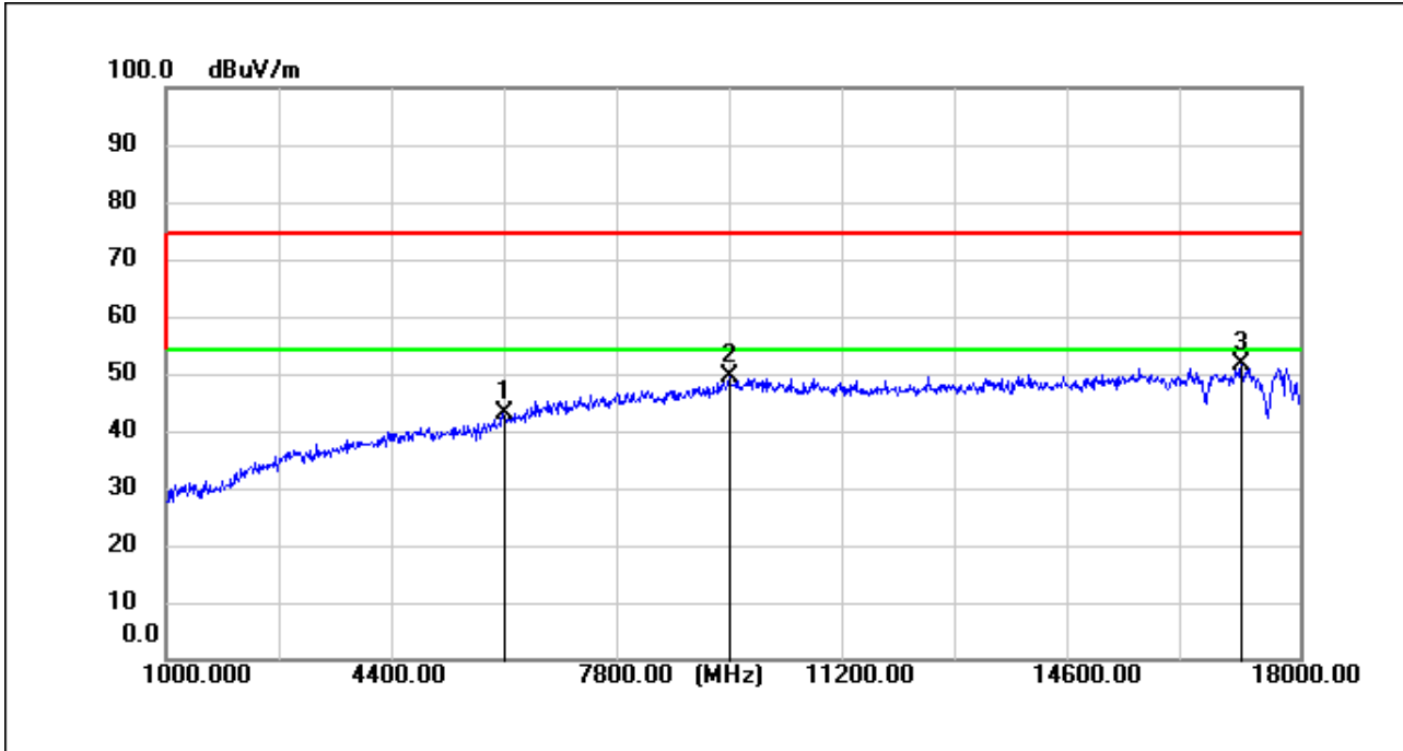
BT_2DH5_TX_CH_78_Horizontal
