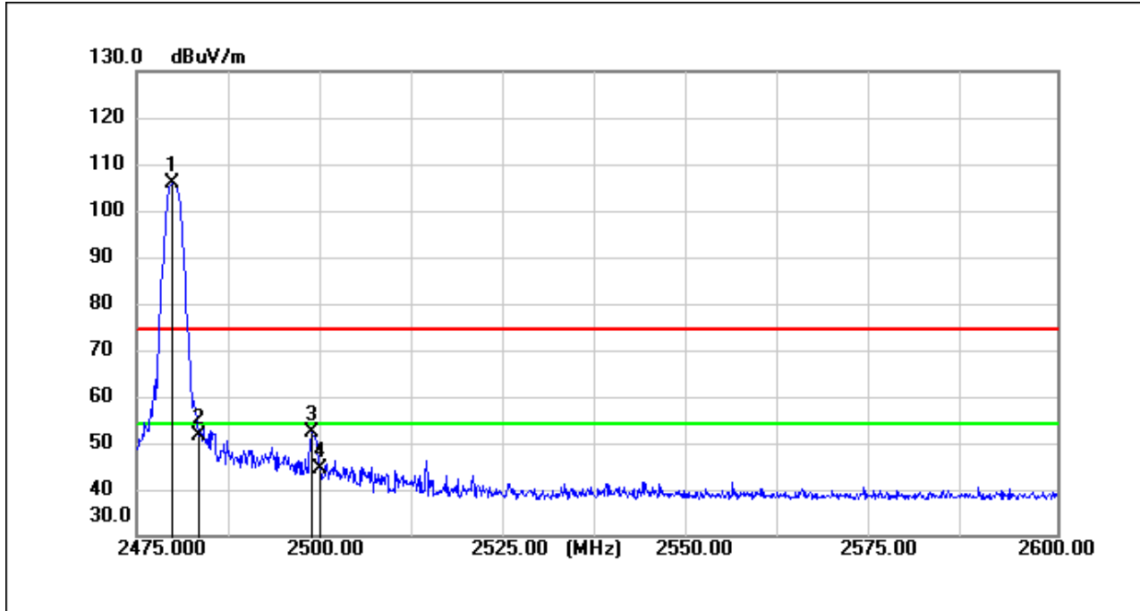
BT_DH5_TX_CH_78_Vertical_Peak
