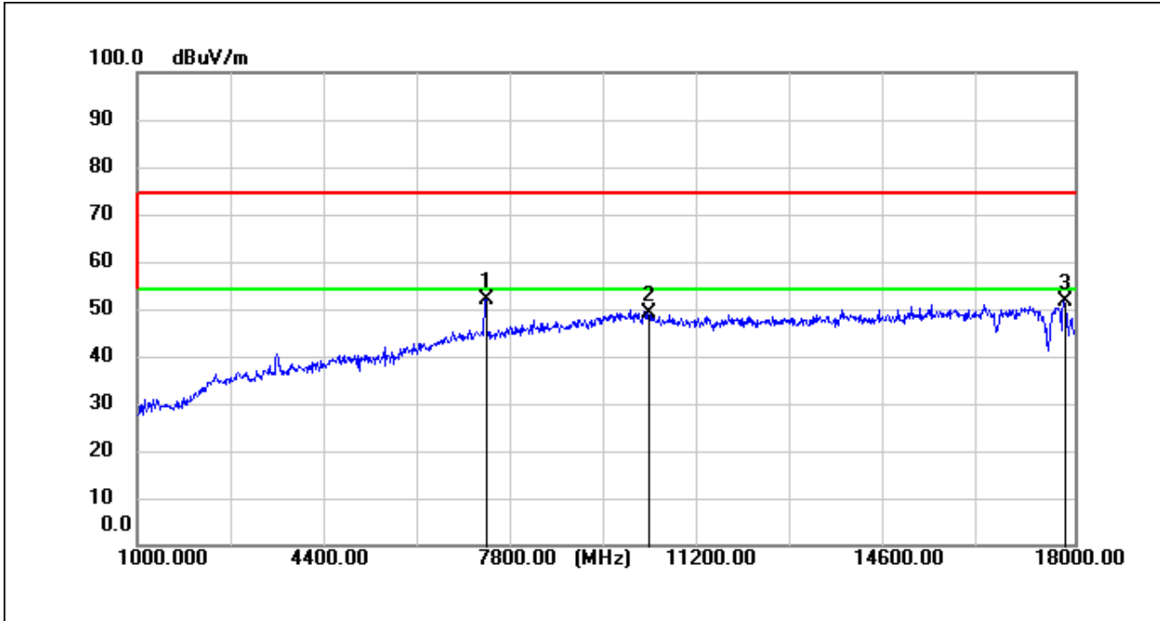
BT_DH5_TX_CH_39_Vertical
