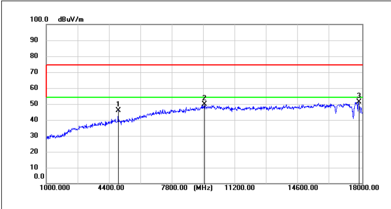
BT_2DH5_TX_CH_39_Vertical
