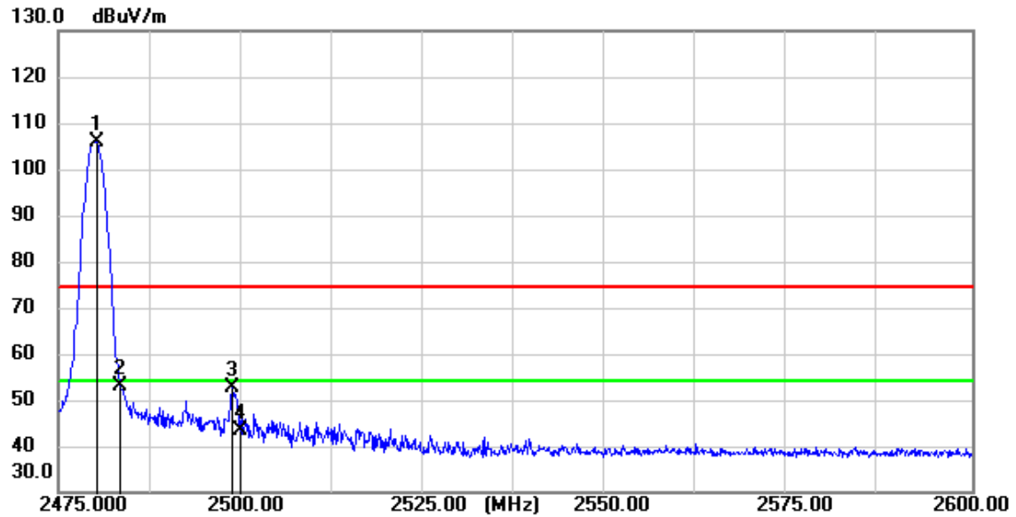
BT_2DH5_TX_CH_78_Horizontal_Peak
