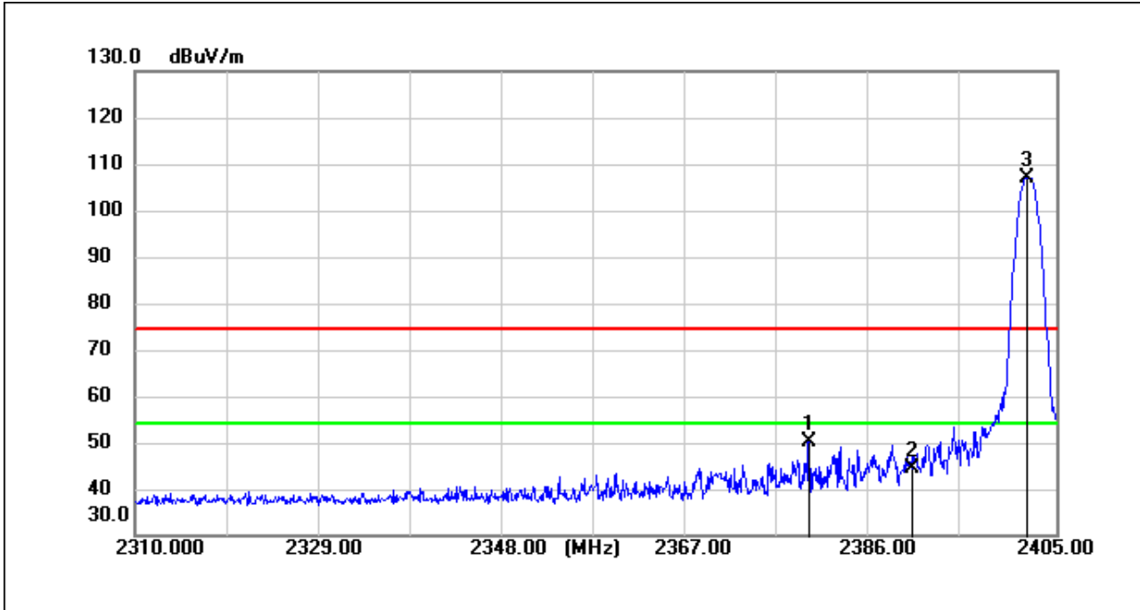
BT_DH5_TX_CH_00_Vertical_Peak
