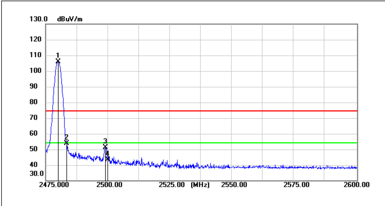
BT_3DH5_TX_CH_78_Horizontal_Peak
