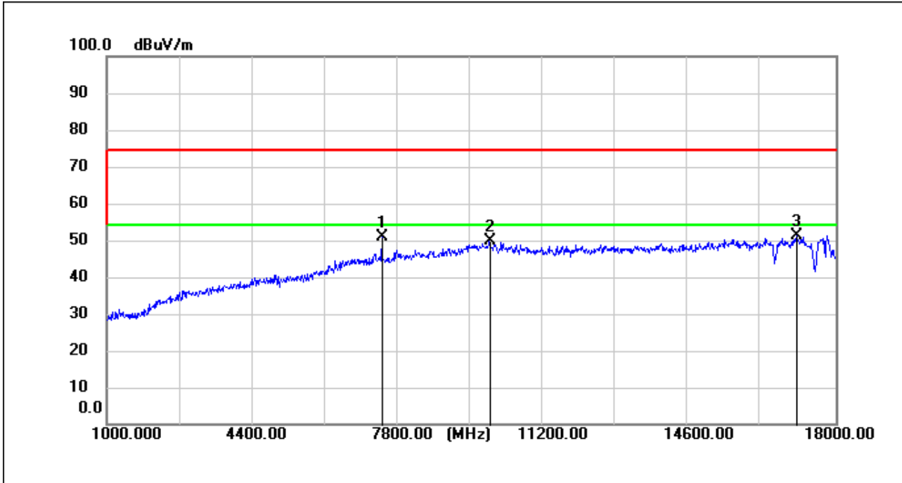
BT_DH5_TX_CH_78_Vertical
