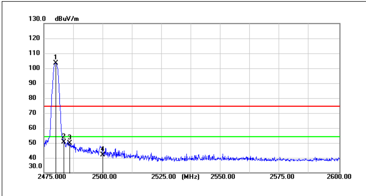
BT_DH5_TX_CH_78_Horizontal_Peak
