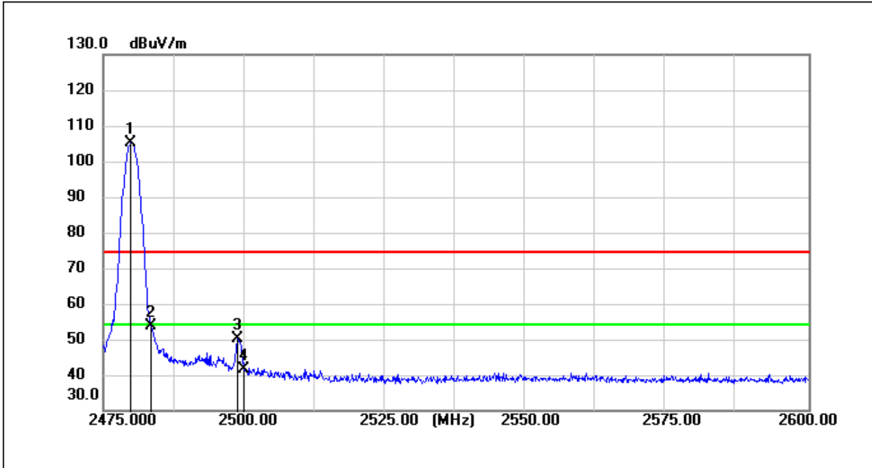
BT_2DH5_TX_CH_78_Vertical_Peak
