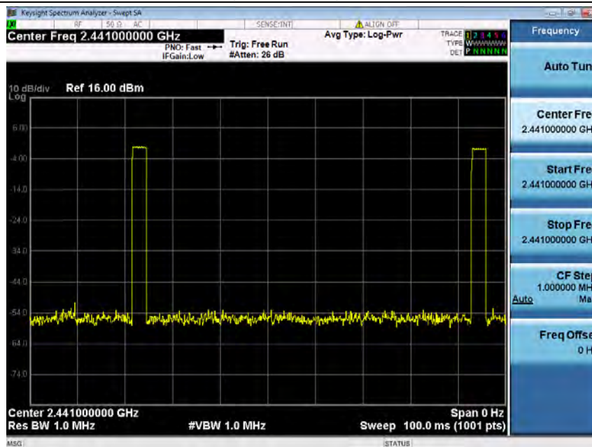
3DH5 on time(Count Pulses)Plot on channel 39
