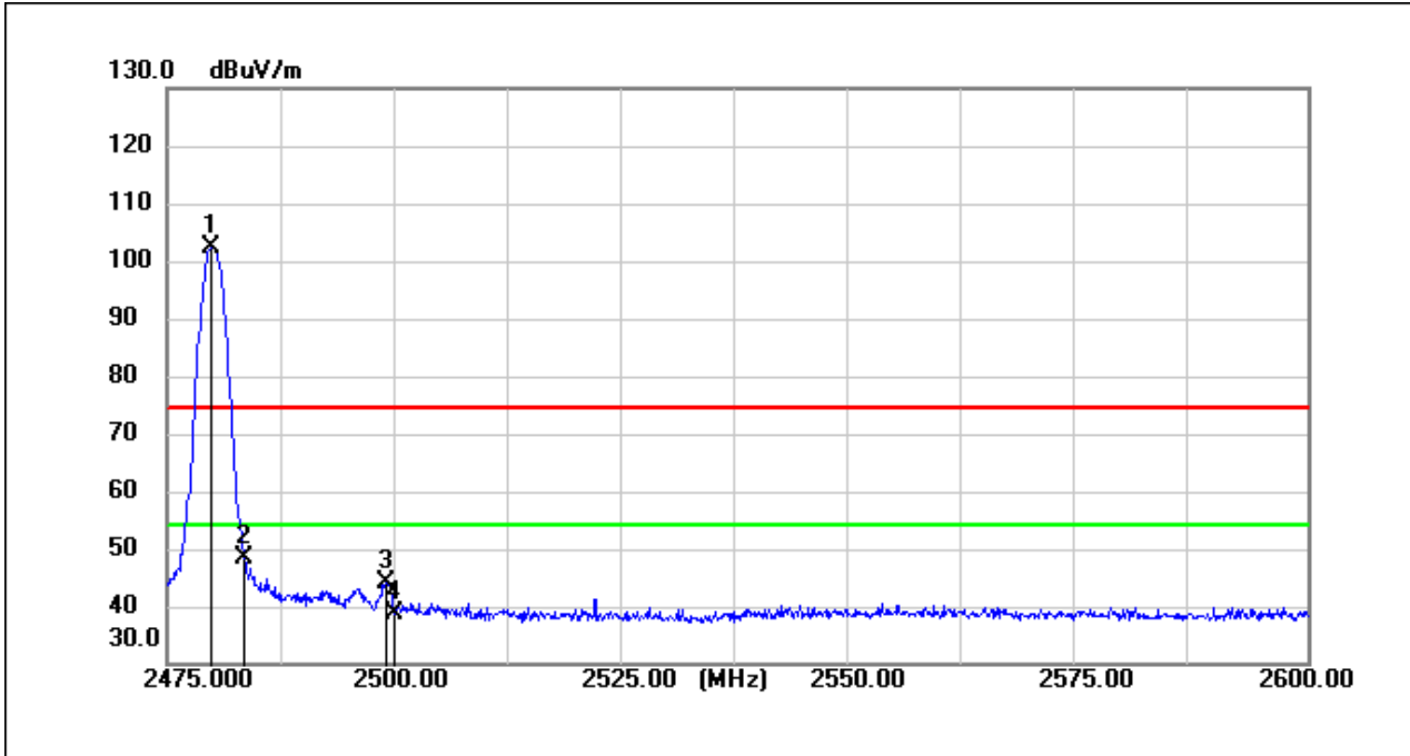
BT_3DH5_TX_CH_78_Horizontal_Peak
