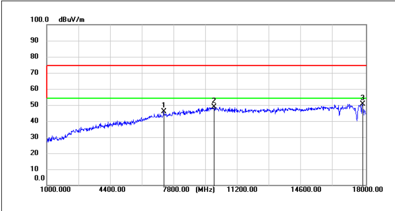
BT_3DH5_TX_CH_39_Vertical
