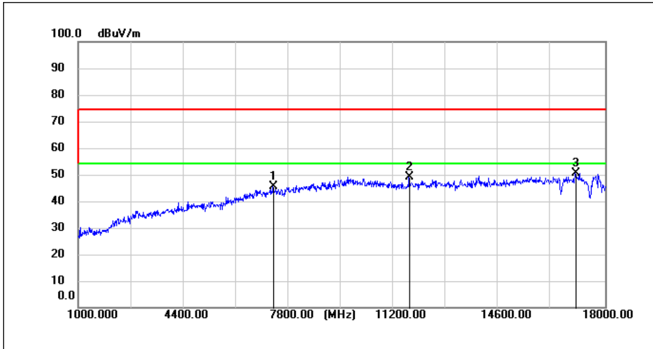
BT_3DH5_TX_CH_78_Horizontal
