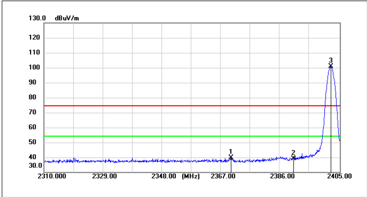
BT_2DH5_TX_CH_00_Horizontal_Peak
