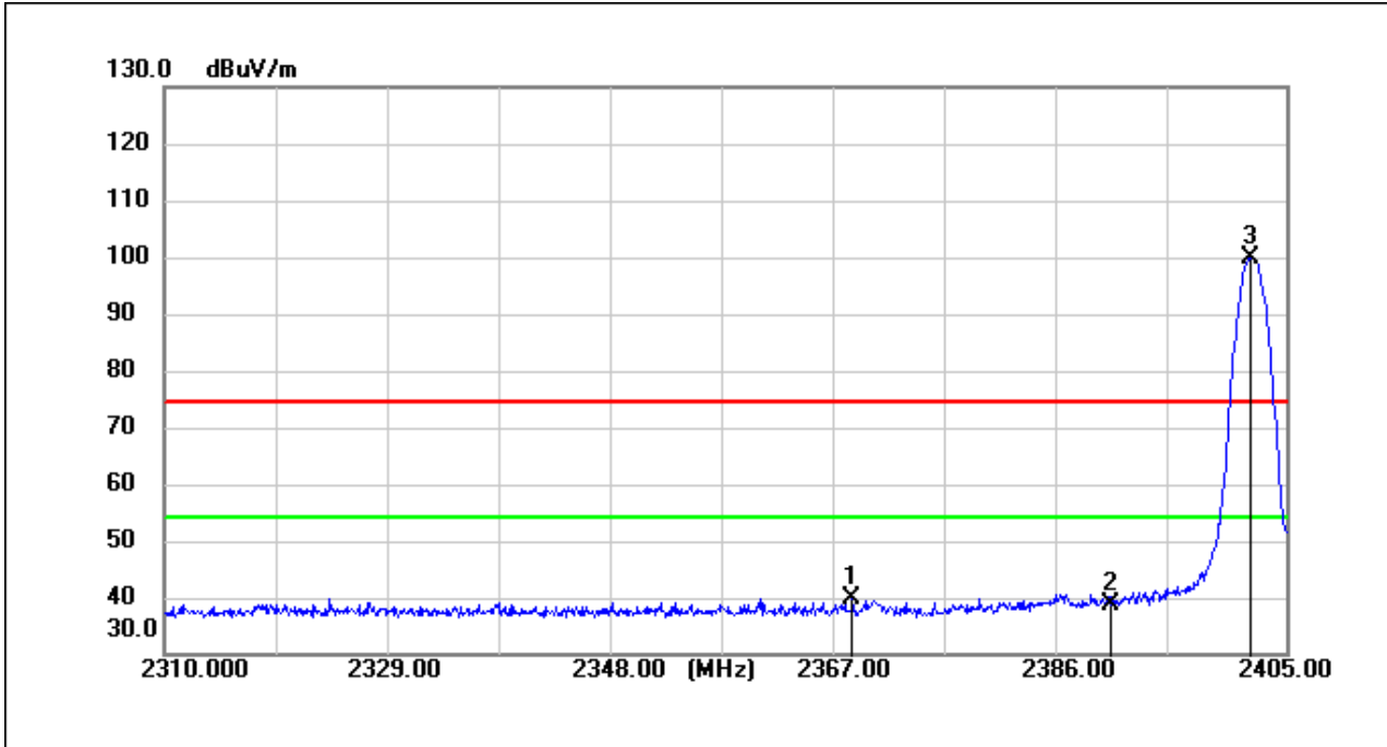
BT_3DH5_TX_CH_00_Horizontal_Peak
