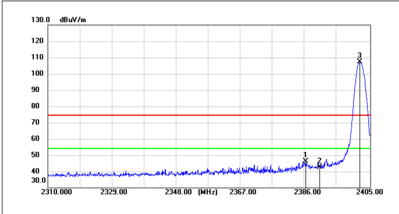
BT_3DH5_TX_CH_00_Horizontal_Peak
