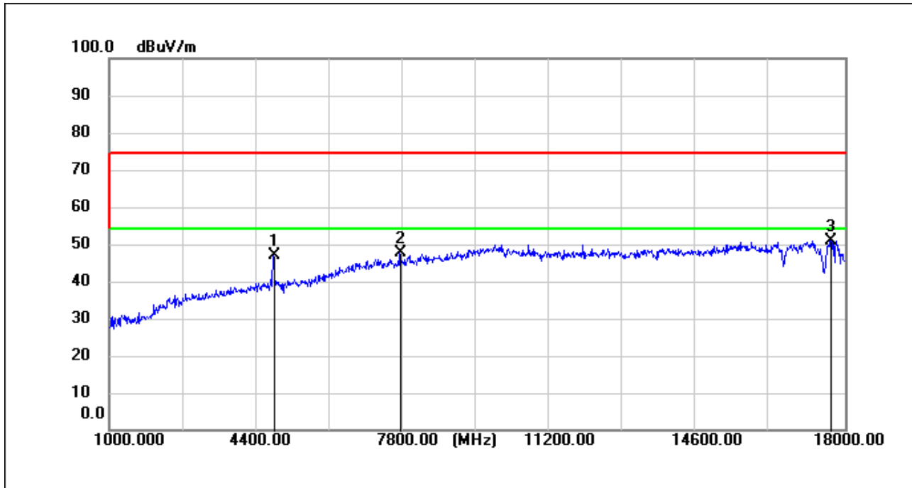
BT_3DH5_TX_CH_00_Horizontal
