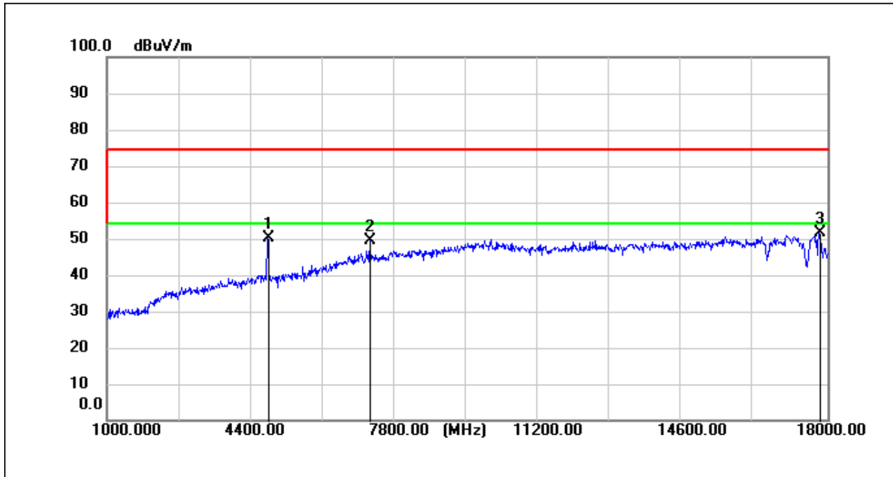
BT_DH5_TX_CH_00_Verical
