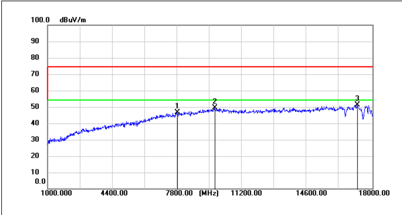
BT_2DH5_TX_CH_78_Vertical
