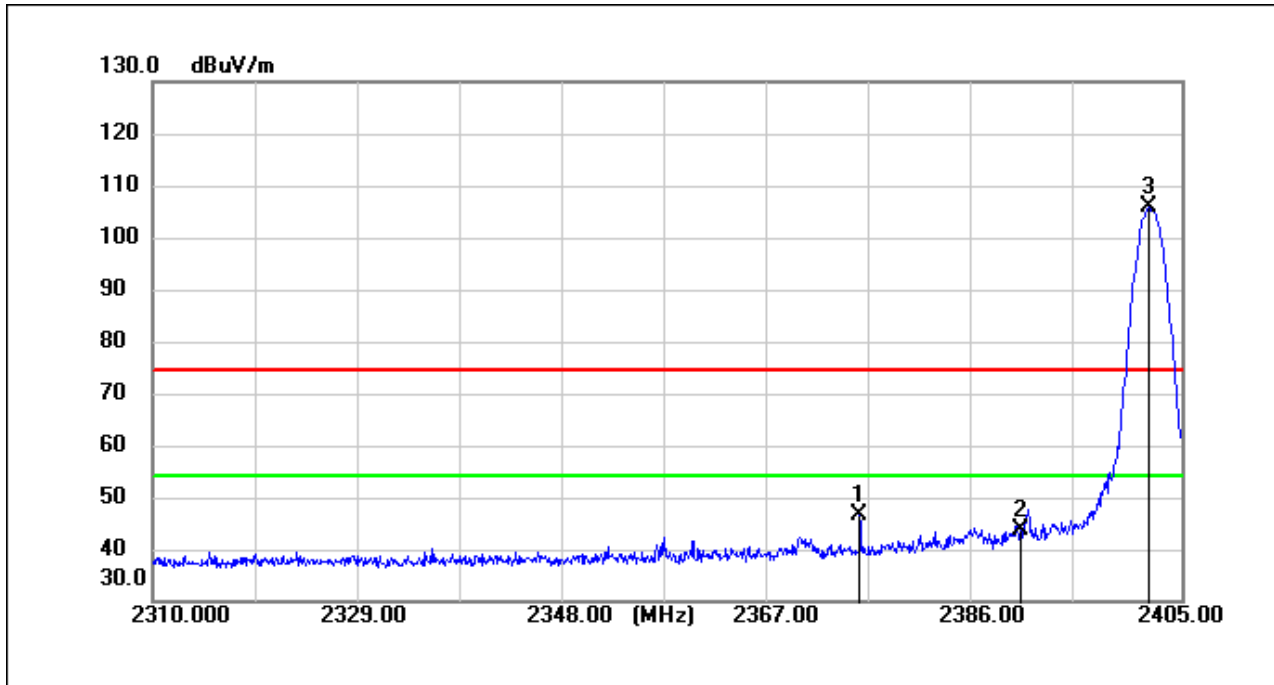
BT_3DH5_TX_CH_00_Vertical_Peak
