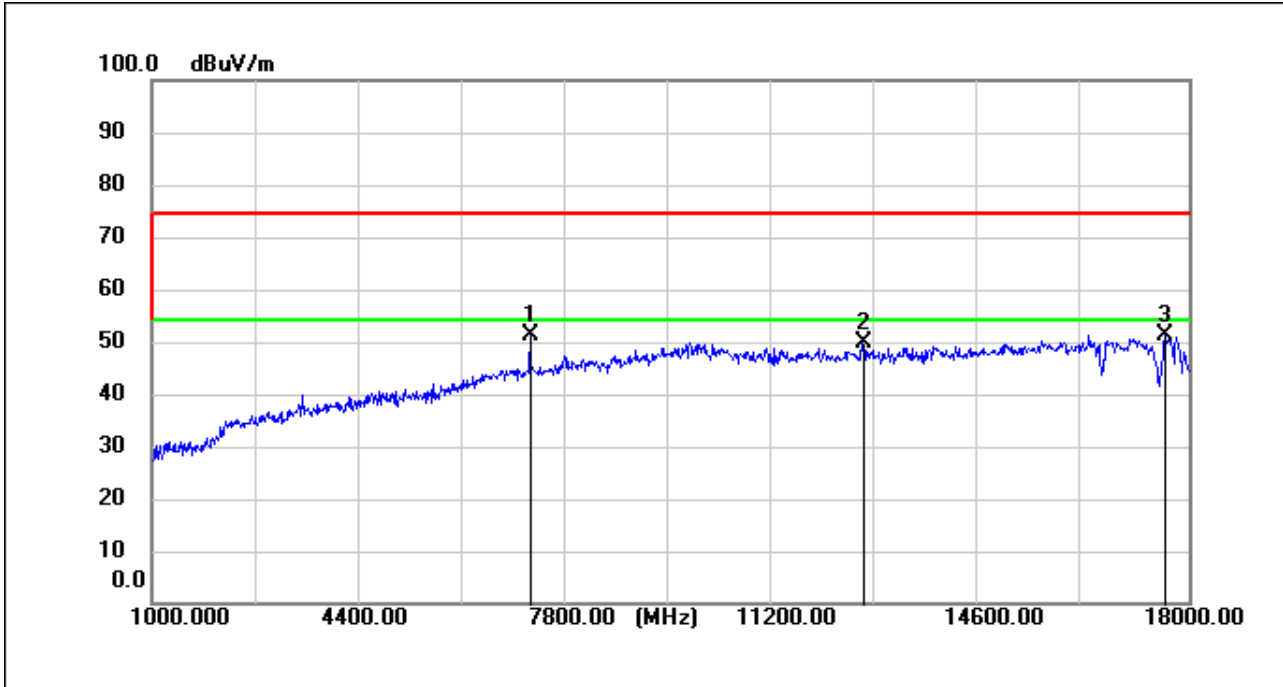
BT_DH5_TX_CH_00_Vertical
