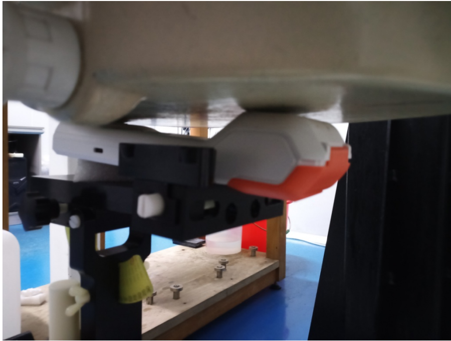
Limb Back1 Setup Photo(0mm)
