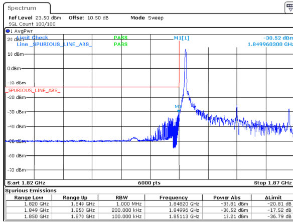
20MHz_Low_16QAM_1@0
