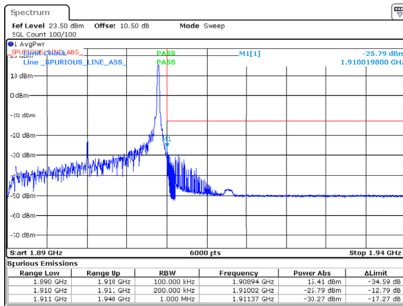
20MHz_High_QPSK_1@99
