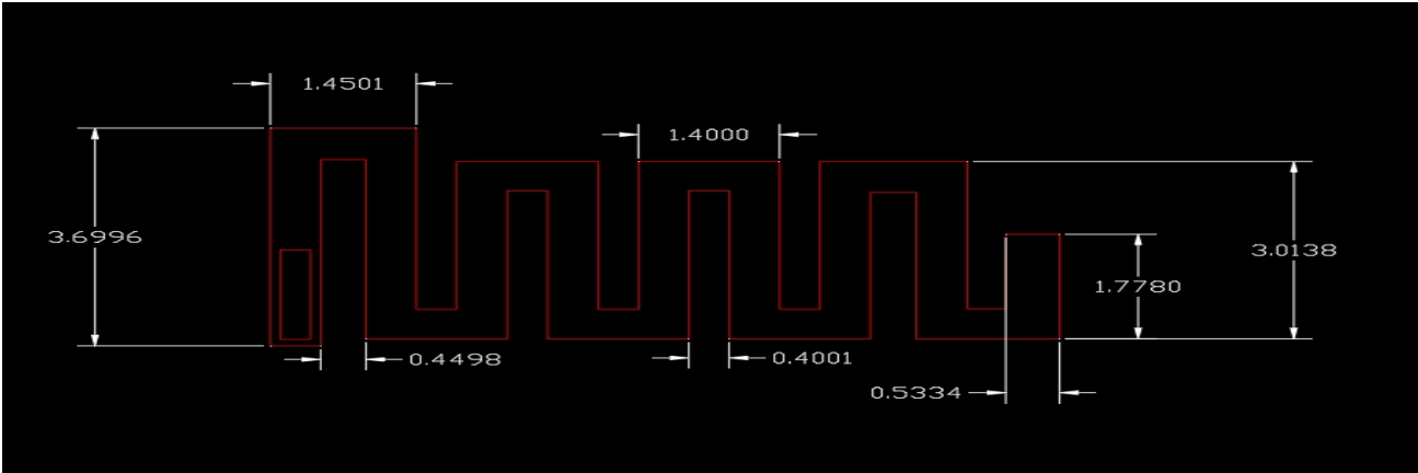
Picture of antenna
