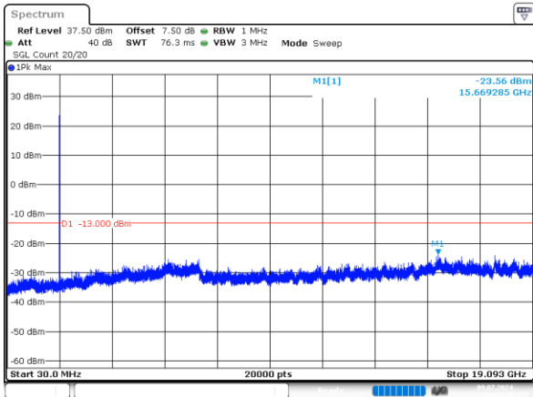
1.4MHz_High_QPSK_6@0 -23.56dBm
