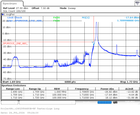
10MHz_Low_16QAM_1@0
