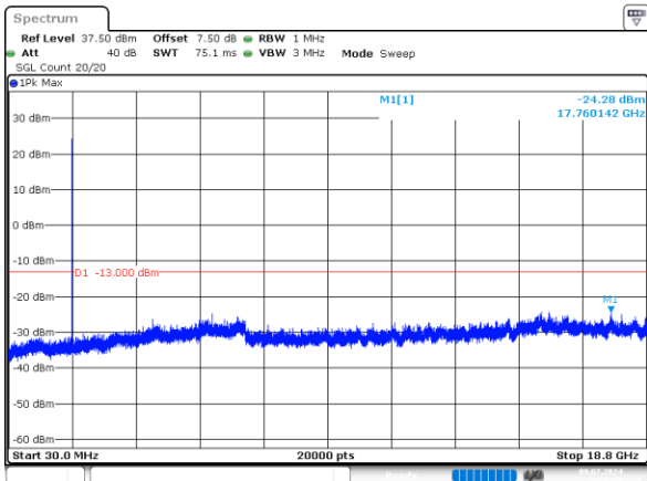
1.4MHz_Middle_QPSK_6@0 -24.28dBm
