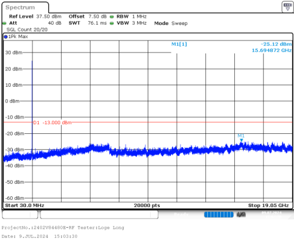
10MHz_High_QPSK_1@0 -25.12dBm
