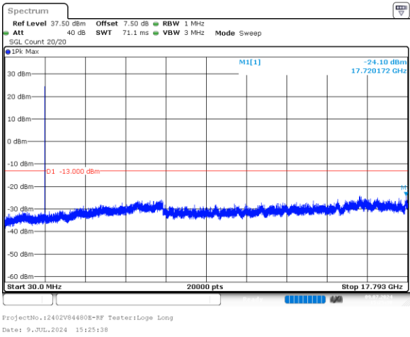
1.4MHz_High_QPSK_1@0 -24.10dBm
