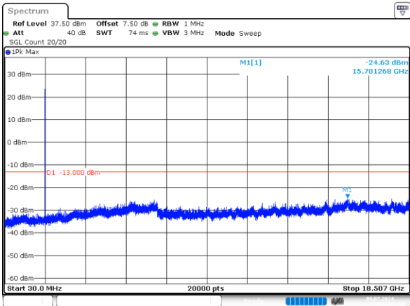
1.4MHz_Low_QPSK_1@0 -24.63dBm
