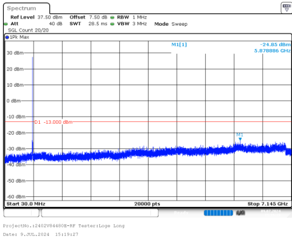
3MHz_High_QPSK_1@0 -24.85dBm
