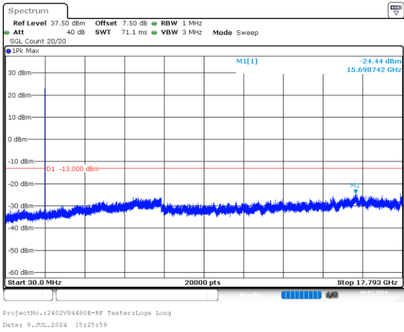
1.4MHz_High_QPSK_6@0 -24.44dBm
