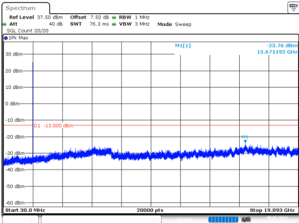
1.4MHz_High_QPSK_1@0 -23.76dBm
