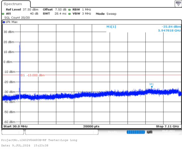
10MHz_High_QPSK_50@0 -25.84dBm
