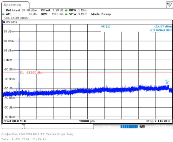
3MHz_High_QPSK_15@0 -25.57dBm
