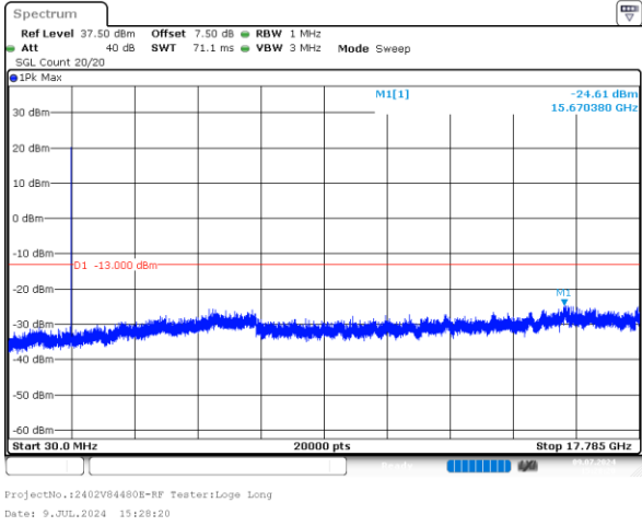
3MHz_High_QPSK_15@0 -24.61dBm
