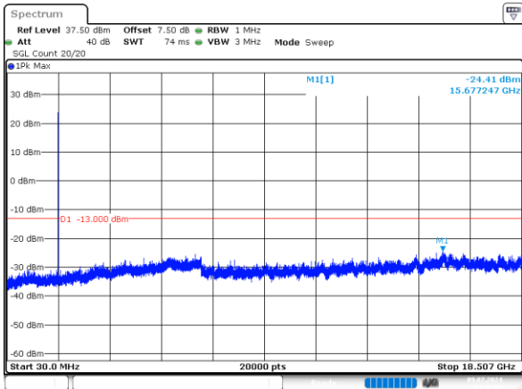
1.4MHz_Low_QPSK_6@0 -24.41dBm
