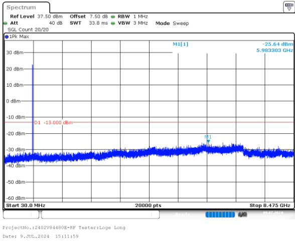
3MHz_High_QPSK_15@0 -25.64dBm
