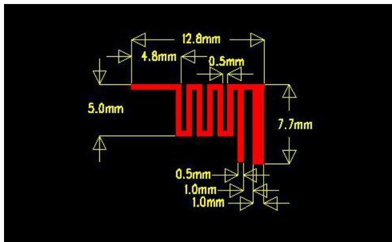
Figure 1 :Keyboard Antenna size
