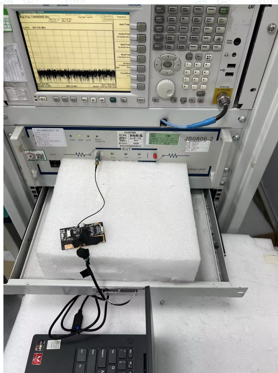
Fig. 4 Conducted Measurement
