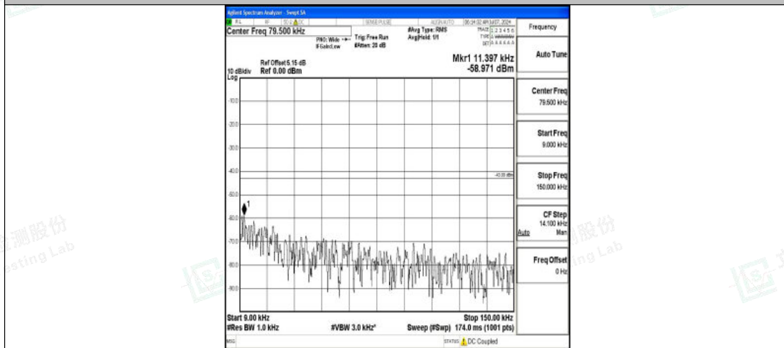
Band4_20MHz_QPSK_20175_1RB#0_0.009~0.15_0.009~0.15
