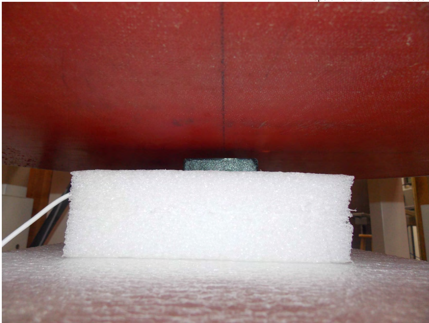
Test Position Left Dongle 5 mm Gap
