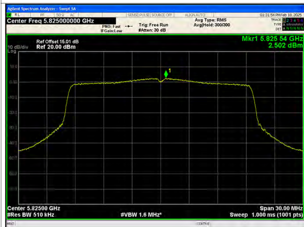
PSD NVNT ax20 5825MHz Ant2 SISO
