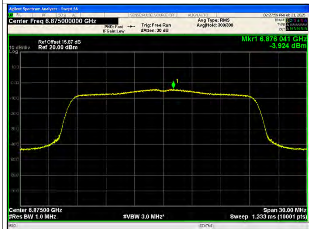
PSD NVNT ax20 6875MHz Ant1 SISO
