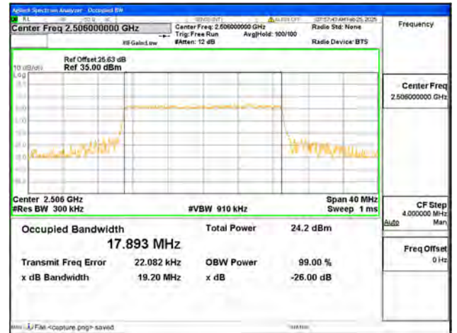
B41 / 20MHz / 256QAM/ Low CH
