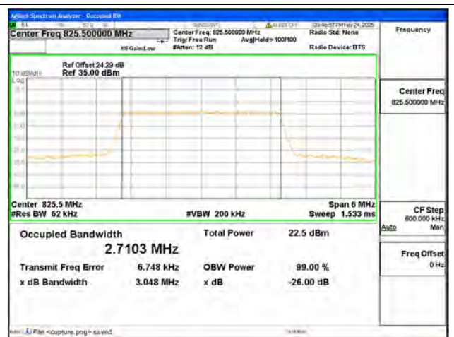
B26 / 3MHz / 16QAM/ Low CH
