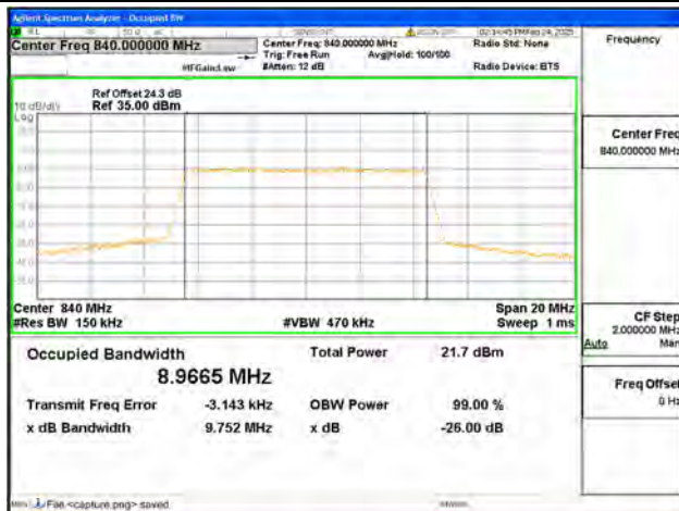
B19 / 10MHz / 64QAM/ High CH
