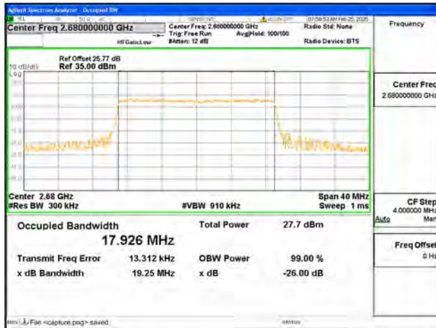
B41 / 20MHz / QPSK/ High CH
