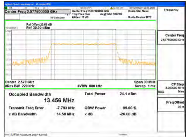
B38 / 15MHz / 256QAM/ Low CH
