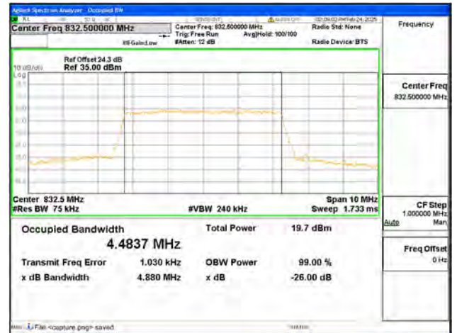
B19 / 5MHz / 256QAM/ Low CH
