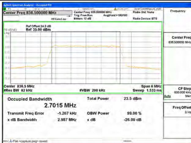
B26 / 3MHz / QPSK/ Mid CH
