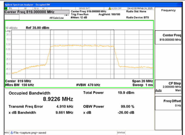
B26 Part90 / 10MHz / 256QAM/ Low CH
