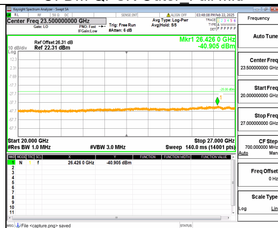
66A_n41 (20GHz-27GHz) 20M DFT-s-OFDM QPSK Inner_1RB_Left Mid
