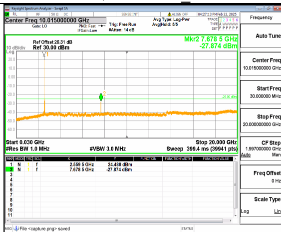
66A_n41 (30MHz-20GHz) 70M DFT-s-OFDM QPSK Inner_1RB_Left Mid
