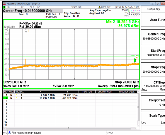
66A_n41 (30MHz-20GHz) 70M DFT-s-OFDM QPSK Inner_1RB_Right Low
