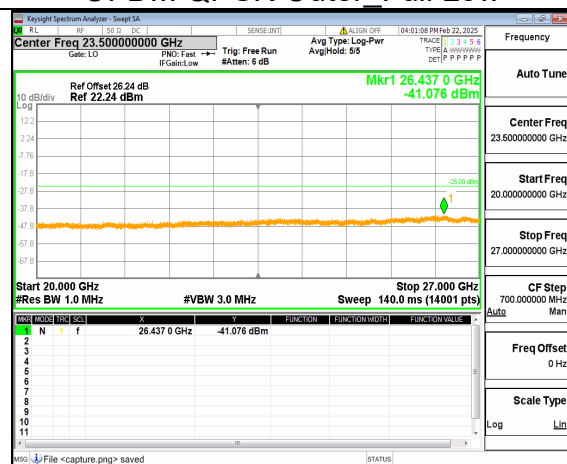
66A_n41 (20GHz-27GHz) 40M DFT-s-OFDM QPSK Inner_1RB_Left Low
