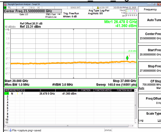
66A_n41 (20GHz-27GHz) 30M DFT-s-OFDM QPSK Outer_Full Mid
