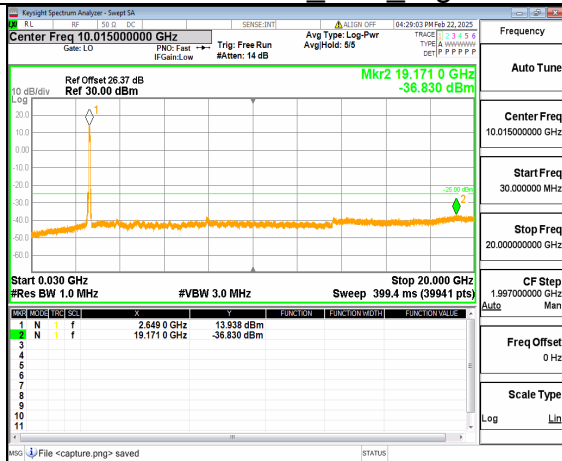
66A_n41 (30MHz-20GHz) 70M DFT-s-OFDM QPSK Outer_Full High
