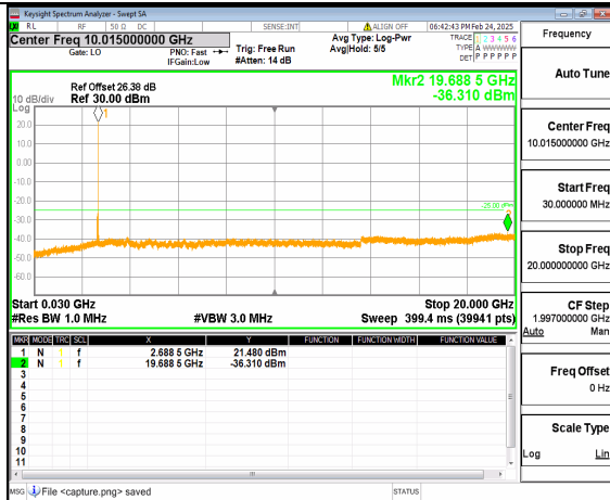
66A_n41 (30MHz-20GHz) 50M DFT-s-OFDM QPSK Inner_1RB_Right High
