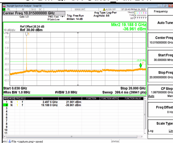
66A_n41 (30MHz-20GHz) 30M DFT-s-OFDM QPSK Inner 1RB Left Low
