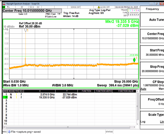
66A_n41 (30MHz-20GHz) 80M DFT-s-OFDM QPSK Inner_1RB_Right Low
