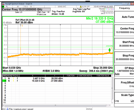
66A_n41 (30MHz-20GHz) 20M DFT-s-OFDM QPSK Inner_1RB_Left_Low
