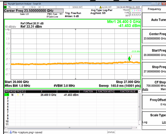
66A_n41 (20GHz-27GHz) 80M DFT-s-OFDM QPSK Outer_Full Mid
