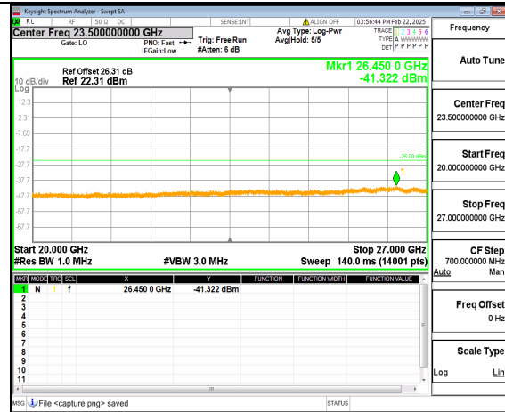
66A_n41 (20GHz-27GHz) 30M DFT-s-OFDM QPSK Inner_1RB_Right Mid
