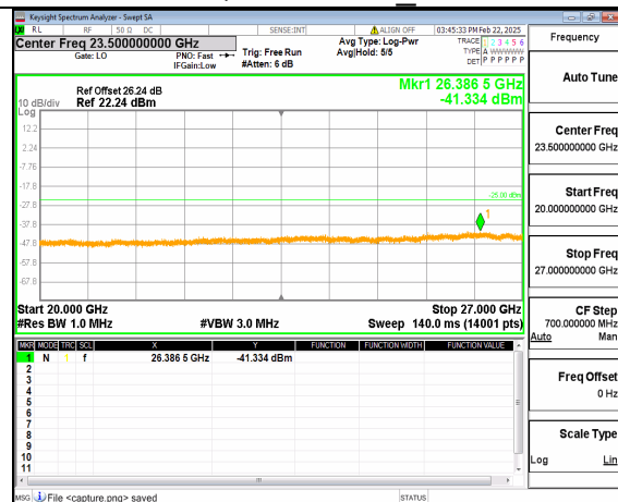
66A_n41 (20GHz-27GHz) 20M DFT-s-OFDM QPSK Inner_1RB_Left_Low
