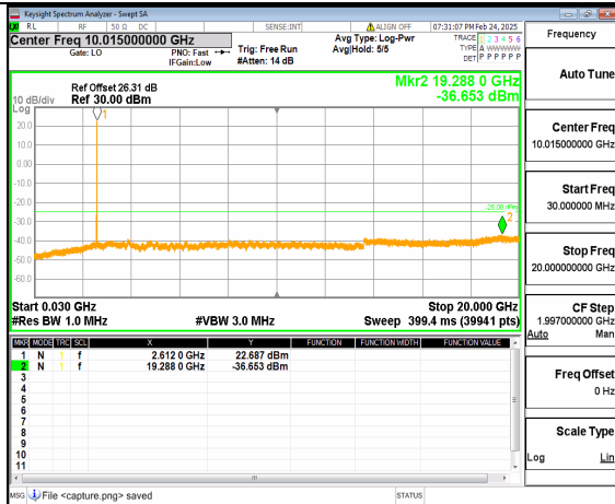
66A_n41 (30MHz-20GHz) 40M DFT-s-OFDM QPSK Inner_1RB_Right Mid
