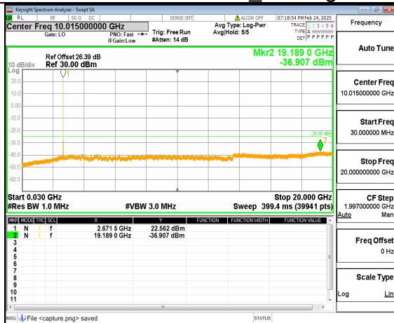
66A_n41 (30MHz-20GHz) 20M DFT-s-OFDM QPSK Inner_1RB_Left High
