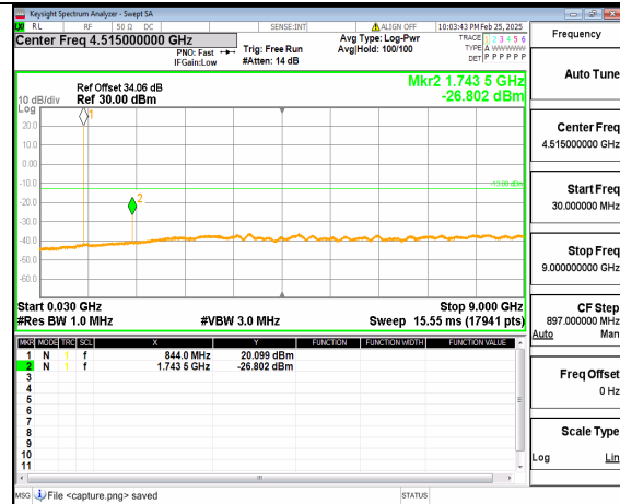
66A_n5 (30MHz-9GHz) 15M DFT-s-OFDM QPSK Inner 1RB Right Mid
