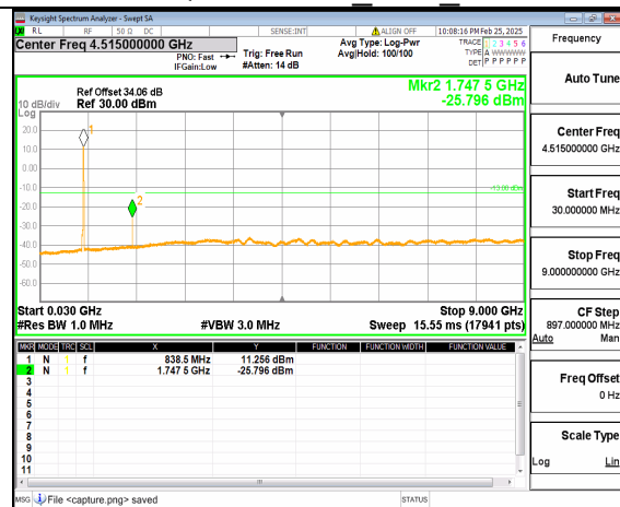
66A_n5 (30MHz-9GHz) 20M DFT-s-OFDM QPSK Outer_Full_High
