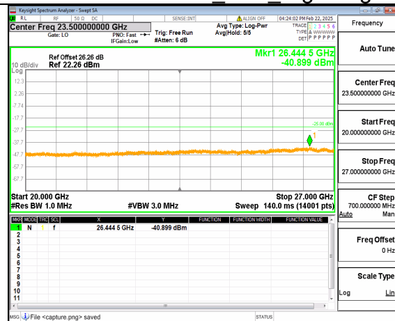
66A_n41 (20GHz-27GHz) 70M DFT-s-OFDM QPSK Outer_Full Low
