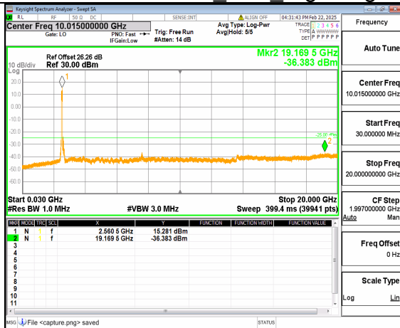
66A_n41 (30MHz-20GHz) 80M DFT-s-OFDM QPSK Outer_Full_Low
