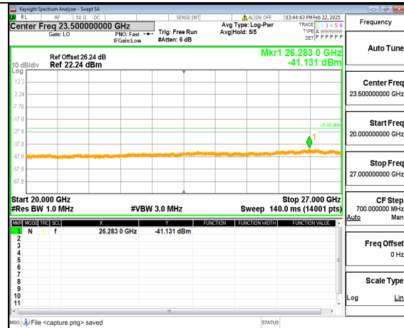
66A_n41 (20GHz-27GHz) 20M DFT-s-OFDM QPSK Outer_Full_Low
