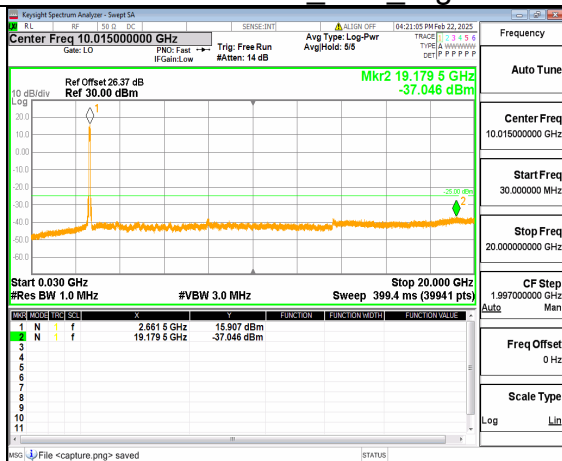
66A_n41 (30MHz-20GHz) 60M DFT-s-OFDM QPSK Outer_Full High
