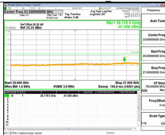
66A_n41 (20GHz-27GHz) 50M DFT-s-OFDM QPSK Inner_1RB_Left Low
