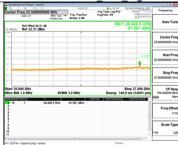
66A_n41 (20GHz-27GHz) 60M DFT-s-OFDM QPSK Outer_Full Mid
