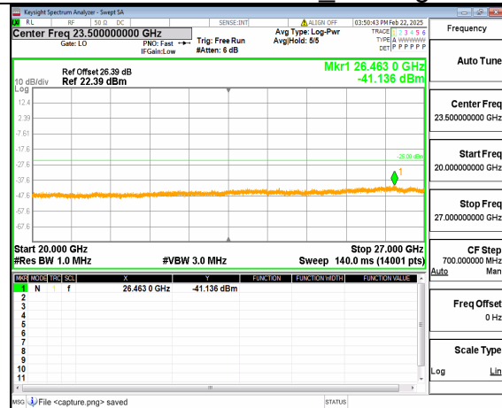
66A_n41 (20GHz-27GHz) 20M DFT-s-OFDM QPSK Inner_1RB_Left High
