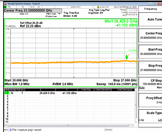
66A_n41 (20GHz-27GHz) 60M DFT-s-OFDM QPSK Inner_1RB_Right Low
