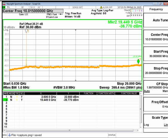
66A_n41 (30MHz-20GHz) 30M DFT-s-OFDM QPSK Inner_1RB_Right Mid
