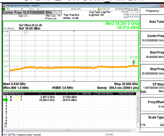
66A_n41 (30MHz-20GHz) 40M DFT-s-OFDM QPSK Inner_1RB_Left Low
