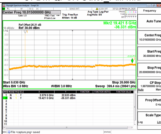
66A_n41 (30MHz-20GHz) 30M DFT-s-OFDM QPSK Inner_1RB_Left Mid
