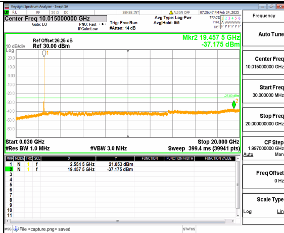
66A_n41 (30MHz-20GHz) 60M DFT-s-OFDM QPSK Inner_1RB_Right Low
