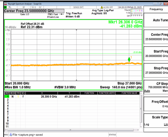
66A_n41 (20GHz-27GHz) 60M DFT-s-OFDM QPSK Inner_1RB_Right Mid
