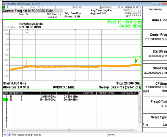
66A_n41 (30MHz-20GHz) 30M DFT-s-OFDM QPSK Inner_1RB_Right High
