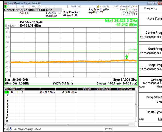
66A_n41 (20GHz-27GHz) 30M DFT-s-OFDM QPSK Outer_Full High
