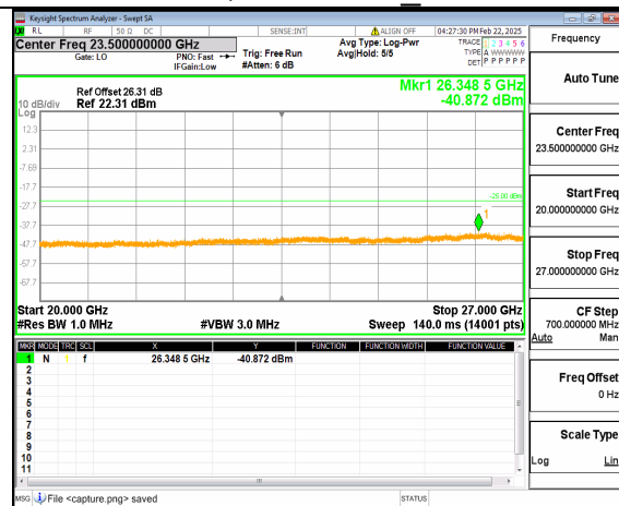
66A_n41 (20GHz-27GHz) 70M DFT-s-OFDM QPSK Inner_1RB_Left Mid
