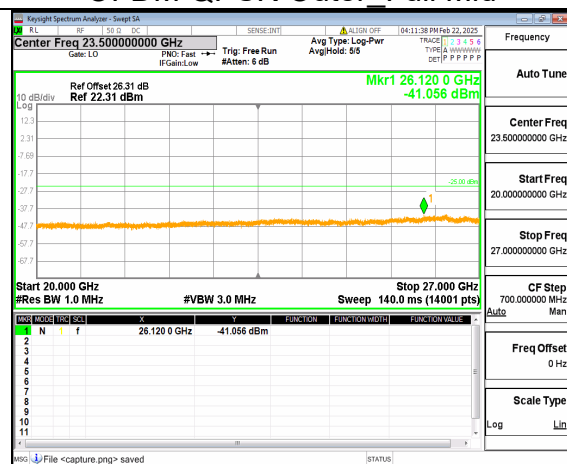
66A_n41 (20GHz-27GHz) 50M DFT-s-OFDM QPSK Inner_1RB_Left Mid
