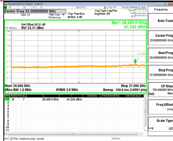
66A_n41 (20GHz-27GHz) 70M DFT-s-OFDM QPSK Inner_1RB_Right Mid
