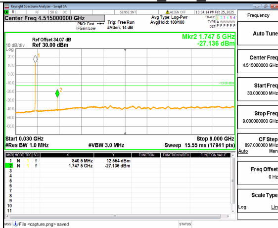
66A_n5 (30MHz-9GHz) 15M DFT-s-OFDM QPSK Outer Full High
