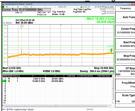
66A_n41 (30MHz-20GHz) 50M DFT-s-OFDM QPSK Inner_1RB_Left High
