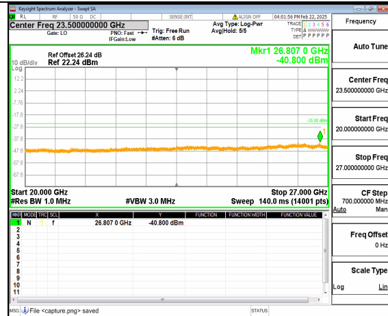
66A_n41 (20GHz-27GHz) 40M DFT-s-OFDM QPSK Inner_1RB_Right Low
