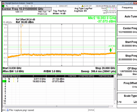
66A_n41 (30MHz-20GHz) 20M DFT-s-OFDM QPSK Outer_Full_Low
