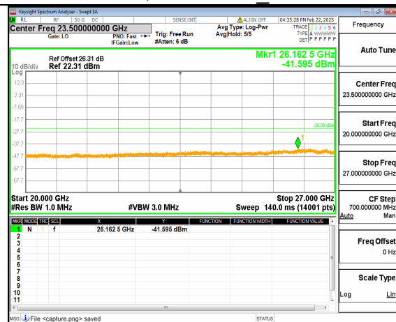
66A_n41 (20GHz-27GHz) 80M DFT-s-OFDM QPSK Inner_1RB_Left Mid
