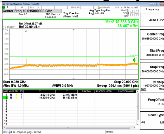
66A_n41 (30MHz-20GHz) 70M DFT-s-OFDM QPSK Inner_1RB_Left High
