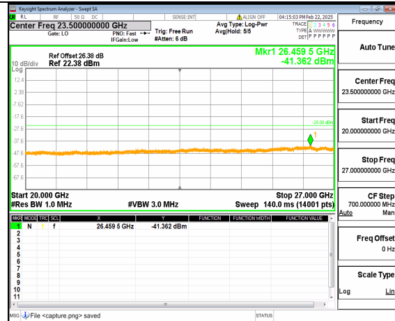
66A_n41 (20GHz-27GHz) 50M DFT-s-OFDM QPSK Inner_1RB_Right High
