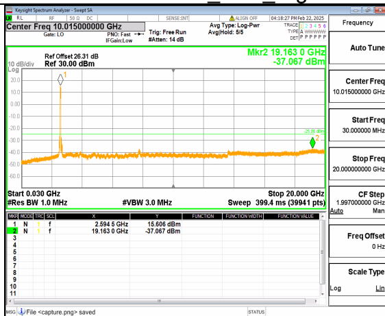
66A_n41 (30MHz-20GHz) 60M DFT-s-OFDM QPSK Outer_Full Mid
