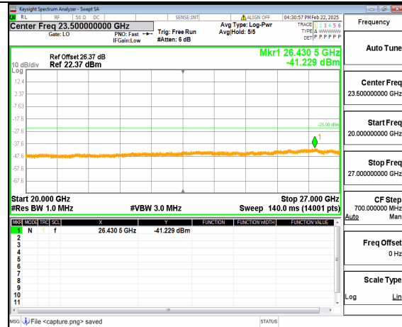
66A_n41 (20GHz-27GHz) 70M DFT-s-OFDM QPSK Inner_1RB_Right_High
