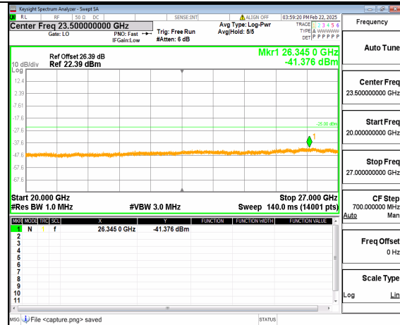
66A_n41 (20GHz-27GHz) 30M DFT-s-OFDM QPSK Inner_1RB_Right High
