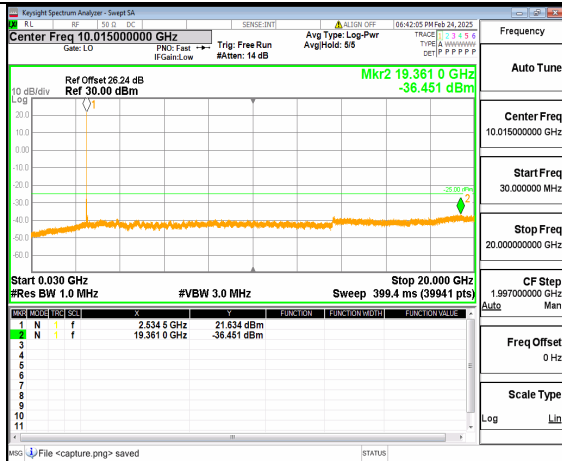
66A_n41 (30MHz-20GHz) 40M DFT-s-OFDM QPSK Inner_1RB_Right Low
