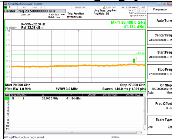
66A_n41 (20GHz-27GHz) 50M DFT-s-OFDM QPSK Outer_Full High
