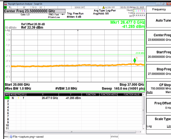
66A_n41 (20GHz-27GHz) 20M DFT-s-OFDM QPSK Inner 1RB Right High
