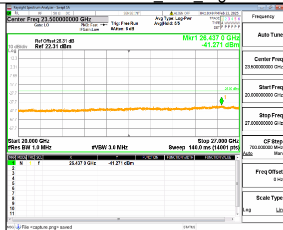
66A_n41 (20GHz-27GHz) 50M DFT-s-OFDM QPSK Outer_Full Mid
