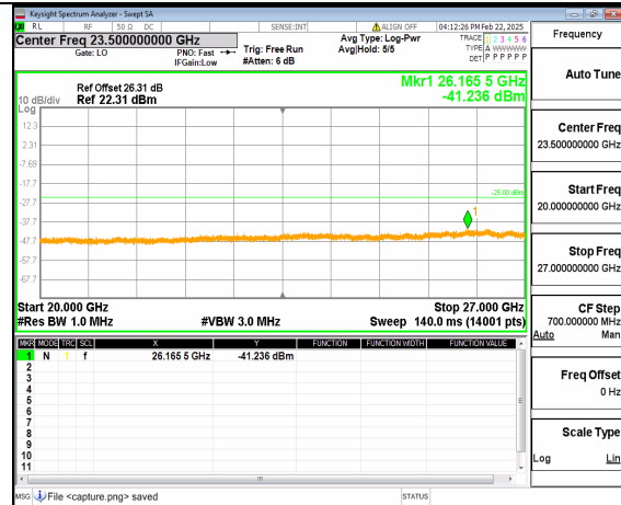
66A_n41 (20GHz-27GHz) 50M DFT-s-OFDM QPSK Inner_1RB_Right Mid
