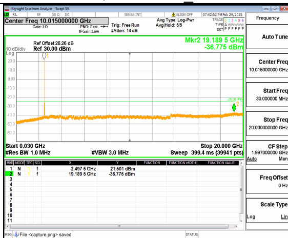
66A_n41 (30MHz-20GHz) 80M DFT-s-OFDM QPSK Inner_1RB_Left_Low
