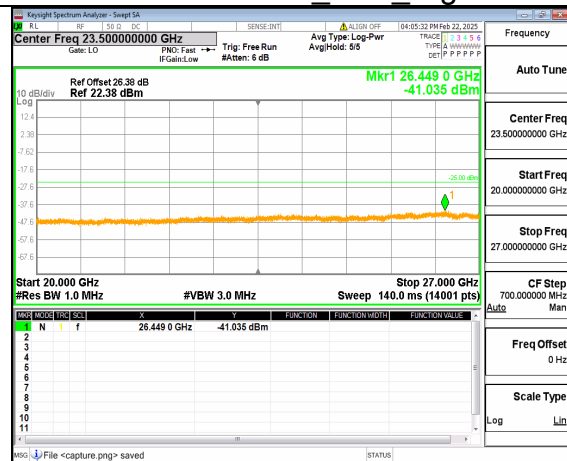
66A_n41 (20GHz-27GHz) 40M DFT-s-OFDM QPSK Outer_Full High
