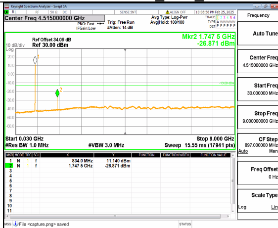
66A_n5 (30MHz-9GHz) 20M DFT-s-OFDM QPSK Outer_Full_Mid
