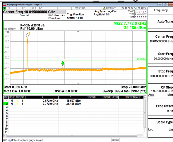
66A_n41 (30MHz-20GHz) 50M DFT-s-OFDM QPSK Outer_Full Mid
