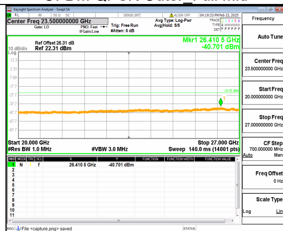
66A_n41 (20GHz-27GHz) 60M DFT-s-OFDM QPSK Inner_1RB_Left Mid
