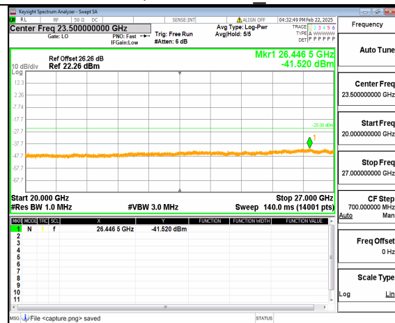
66A_n41 (20GHz-27GHz) 80M DFT-s-OFDM QPSK Inner_1RB_Left_Low
