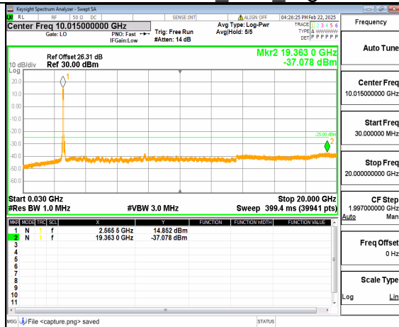
66A_n41 (30MHz-20GHz) 70M DFT-s-OFDM QPSK Outer_Full Mid
