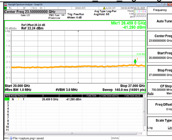
66A_n41 (20GHz-27GHz) 30M DFT-s-OFDM QPSK Outer Full Low
