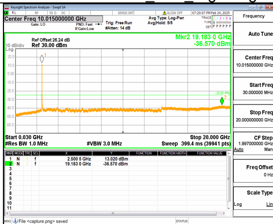
66A_n41 (30MHz-20GHz) 30M DFT-s-OFDM QPSK Outer Full Low
