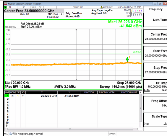
66A_n41 (20GHz-27GHz) 30M DFT-s-OFDM QPSK Inner_1RB_Right Low
