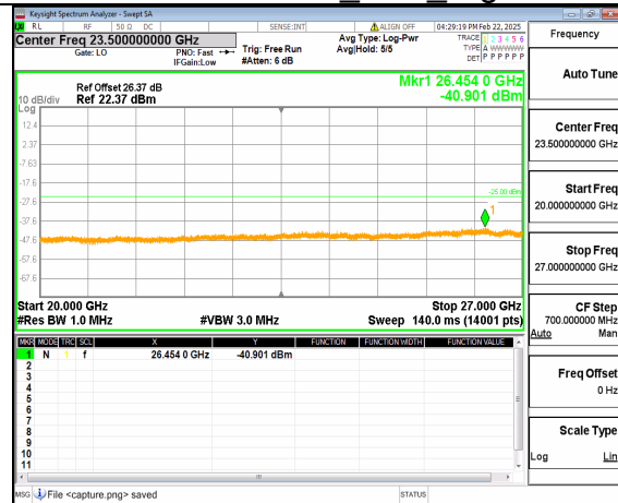
66A_n41 (20GHz-27GHz) 70M DFT-s-OFDM QPSK Outer_Full High
