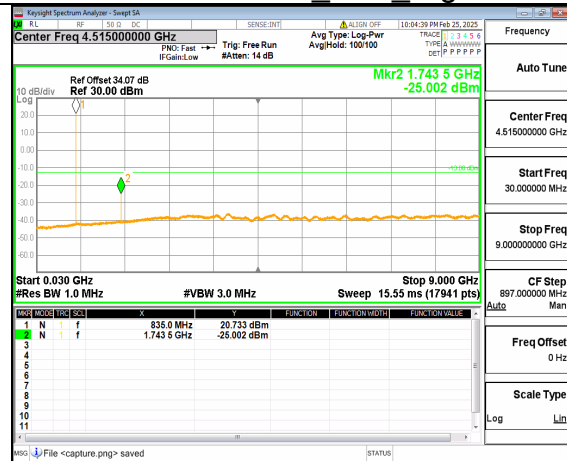
66A_n5 (30MHz-9GHz) 15M DFT-s-OFDM QPSK Inner 1RB Left High
