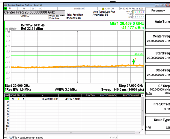
66A_n41 (20GHz-27GHz) 40M DFT-s-OFDM QPSK Inner_1RB_Left Mid
