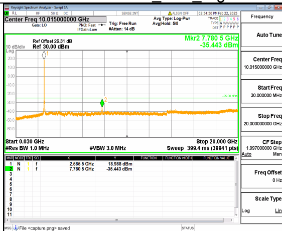
66A_n41 (30MHz-20GHz) 30M DFT-s-OFDM QPSK Outer_Full Mid
