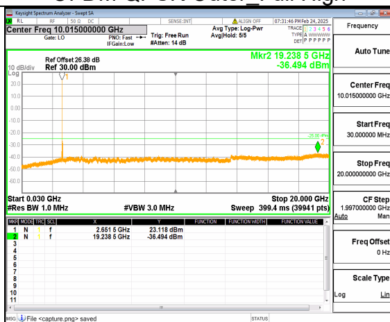
66A_n41 (30MHz-20GHz) 40M DFT-s-OFDM QPSK Inner_1RB_Left High
