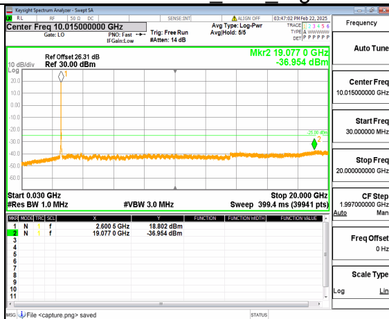
66A_n41 (30MHz-20GHz) 20M DFT-s-OFDM QPSK Outer_Full Mid
