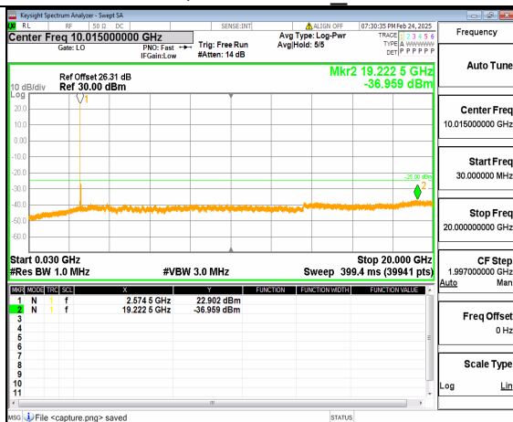
66A_n41 (30MHz-20GHz) 40M DFT-s-OFDM QPSK Inner_1RB_Left Mid
