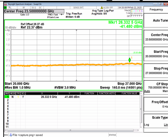
66A_n41 (20GHz-27GHz) 70M DFT-s-OFDM QPSK Inner_1RB_Left High
