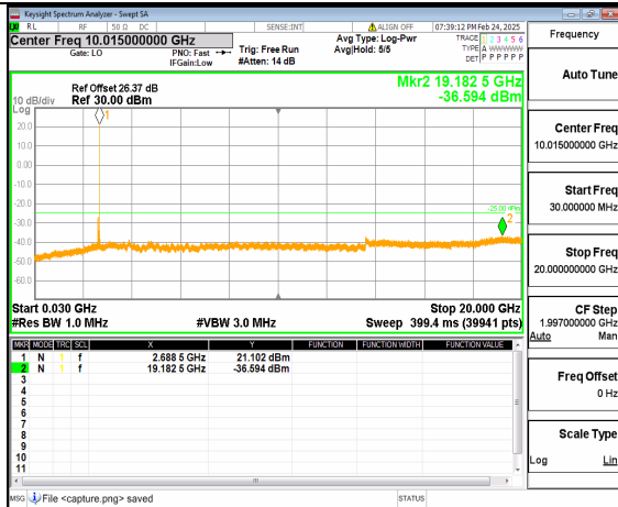
66A_n41 (30MHz-20GHz) 60M DFT-s-OFDM QPSK Inner_1RB_Right High
