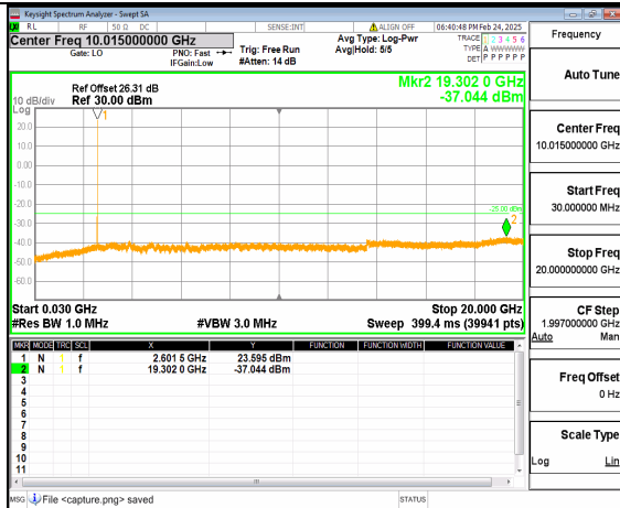
66A_n41 (30MHz-20GHz) 20M DFT-s-OFDM QPSK Inner_1RB_Right Mid
