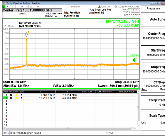
66A_n41 (30MHz-20GHz) 30M DFT-s-OFDM QPSK Outer_Full High
