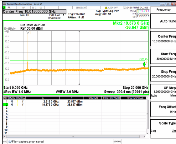
66A_n41 (30MHz-20GHz) 50M DFT-s-OFDM QPSK Inner_1RB_Right Mid
