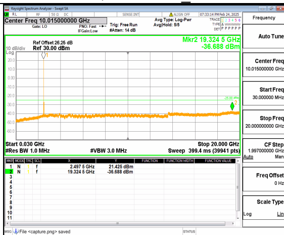
66A_n41 (30MHz-20GHz) 50M DFT-s-OFDM QPSK Inner_1RB_Left Low
