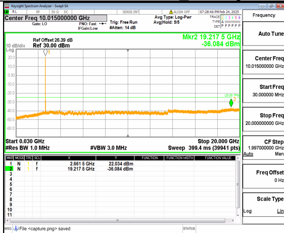
66A_n41 (30MHz-20GHz) 30M DFT-s-OFDM QPSK Inner_1RB_Left High
