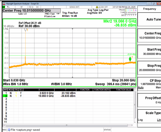
66A_n41 (30MHz-20GHz) 60M DFT-s-OFDM QPSK Inner_1RB_Right Mid
