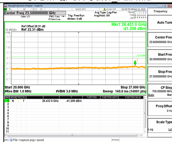
66A_n41 (20GHz-27GHz) 30M DFT-s-OFDM QPSK Inner_1RB_Left Mid
