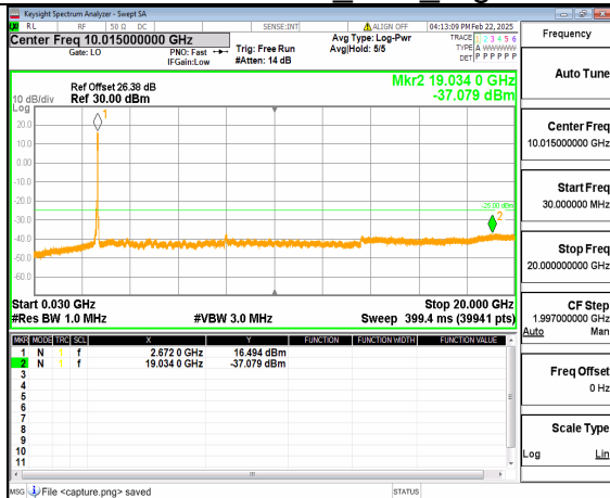
66A_n41 (30MHz-20GHz) 50M DFT-s-OFDM QPSK Outer_Full High
