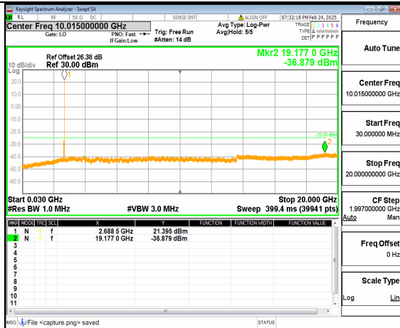
66A_n41 (30MHz-20GHz) 40M DFT-s-OFDM QPSK Inner_1RB_Right High
