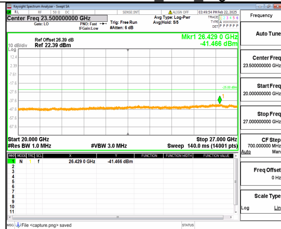
66A_n41 (20GHz-27GHz) 20M DFT-s-OFDM QPSK Outer_Full High
