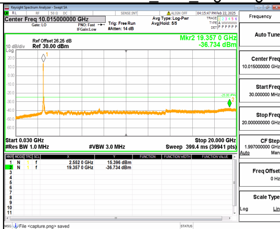
66A_n41 (30MHz-20GHz) 60M DFT-s-OFDM QPSK Outer_Full Low
