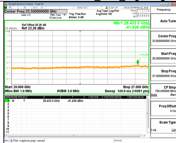
66A_n41 (20GHz-27GHz) 80M DFT-s-OFDM QPSK Outer_Full_Low
