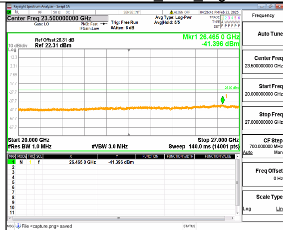
66A_n41 (20GHz-27GHz) 70M DFT-s-OFDM QPSK Outer_Full Mid
