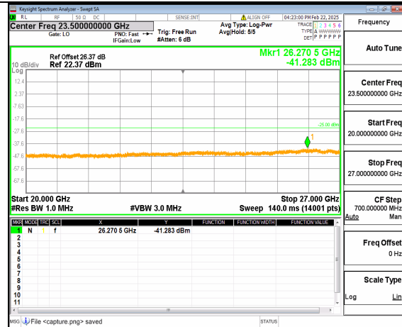
66A_n41 (20GHz-27GHz) 60M DFT-s-OFDM QPSK Inner_1RB_Right High
