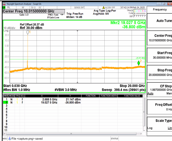
66A_n41 (30MHz-20GHz) 70M DFT-s-OFDM QPSK Inner_1RB_Right_High
