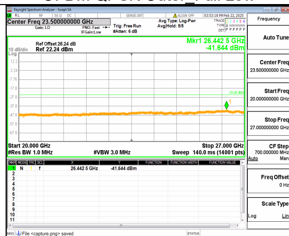
66A_n41 (20GHz-27GHz) 30M DFT-s-OFDM QPSK Inner 1RB Left Low
