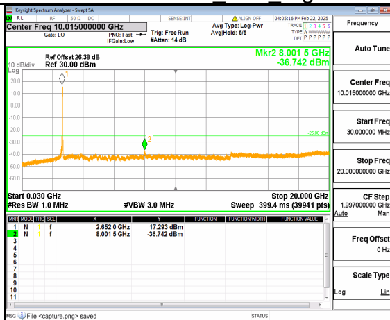
66A_n41 (30MHz-20GHz) 40M DFT-s-OFDM QPSK Outer_Full High
