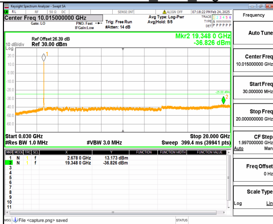
66A_n41 (30MHz-20GHz) 20M DFT-s-OFDM QPSK Outer_Full High
