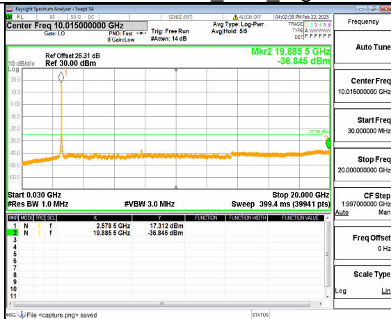
66A_n41 (30MHz-20GHz) 40M DFT-s-OFDM QPSK Outer_Full Mid
