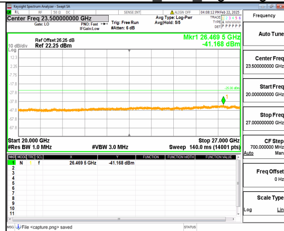
66A_n41 (20GHz-27GHz) 50M DFT-s-OFDM QPSK Outer_Full Low
