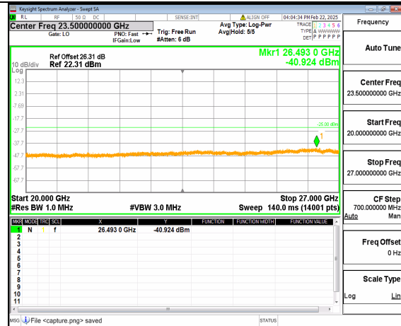
66A_n41 (20GHz-27GHz) 40M DFT-s-OFDM QPSK Inner_1RB_Right Mid
