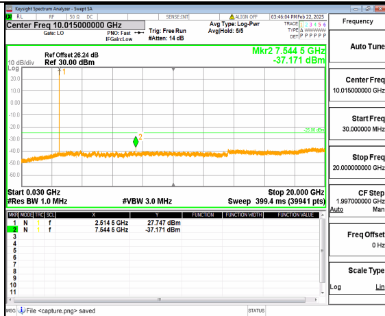
66A_n41 (30MHz-20GHz) 20M DFT-s-OFDM QPSK Inner_1RB_Right Low
