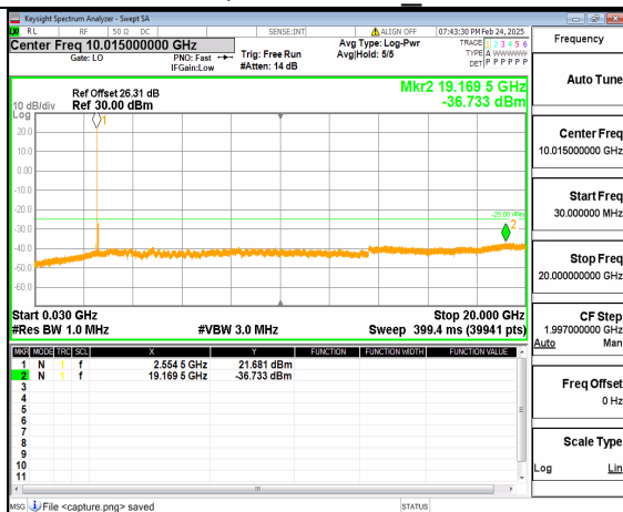
66A_n41 (30MHz-20GHz) 80M DFT-s-OFDM QPSK Inner_1RB_Left Mid
