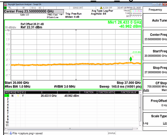
66A_n41 (20GHz-27GHz) 20M DFT-s-OFDM QPSK Outer_Full Mid
