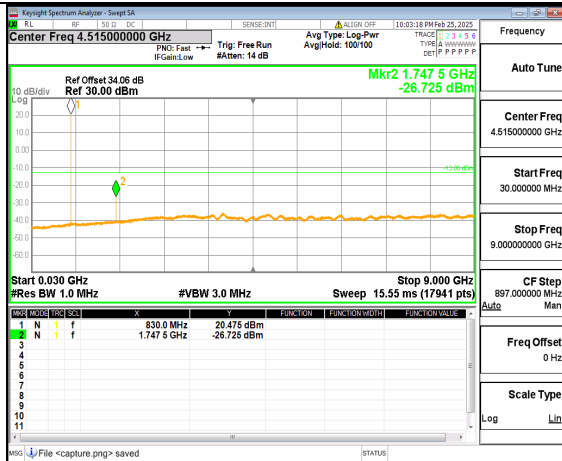
66A_n5 (30MHz-9GHz) 15M DFT-s-OFDM QPSK Inner 1RB Left Mid
