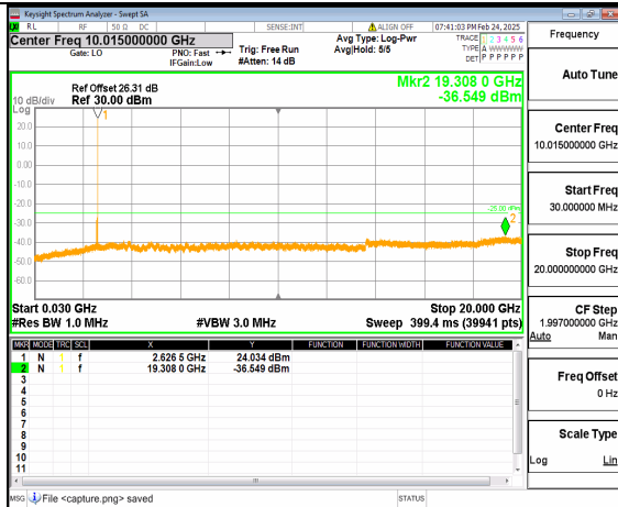
66A_n41 (30MHz-20GHz) 70M DFT-s-OFDM QPSK Inner_1RB_Right Mid
