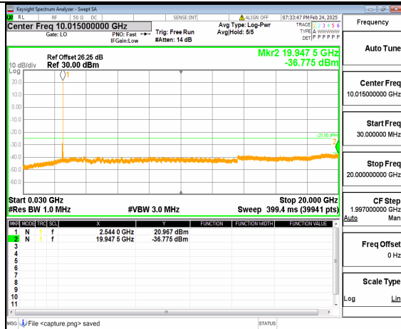
66A_n41 (30MHz-20GHz) 50M DFT-s-OFDM QPSK Inner_1RB_Right Low
