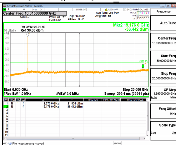
66A_n41 (30MHz-20GHz) 50M DFT-s-OFDM QPSK Inner_1RB_Left Mid
