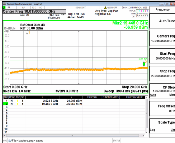
66A_n41 (30MHz-20GHz) 30M DFT-s-OFDM QPSK Inner_1RB_Right Low
