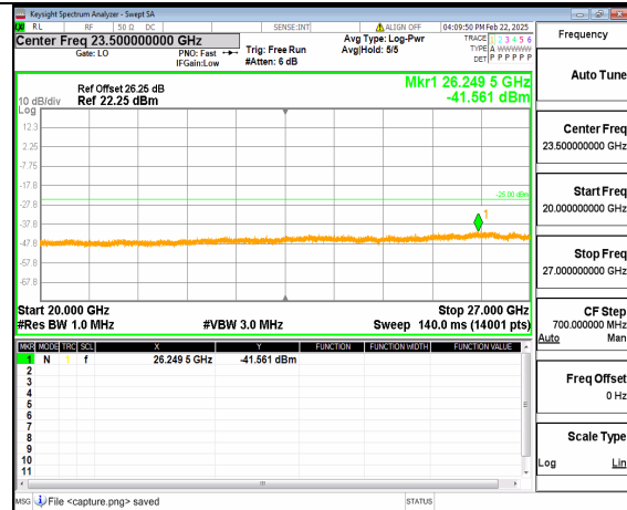
66A_n41 (20GHz-27GHz) 50M DFT-s-OFDM QPSK Inner_1RB_Right Low
