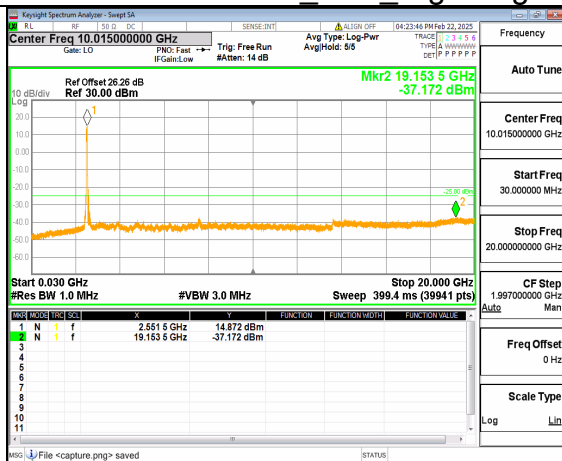
66A_n41 (30MHz-20GHz) 70M DFT-s-OFDM QPSK Outer_Full Low
