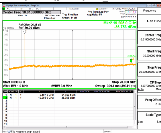
66A_n41 (30MHz-20GHz) 70M DFT-s-OFDM QPSK Inner_1RB_Left Low
