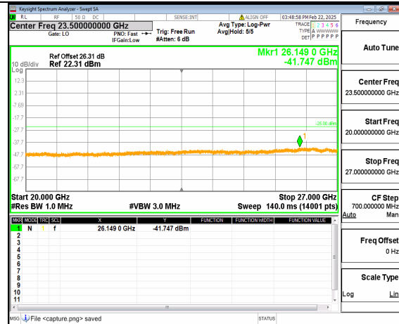
66A_n41 (20GHz-27GHz) 20M DFT-s-OFDM QPSK Inner_1RB_Right Mid
