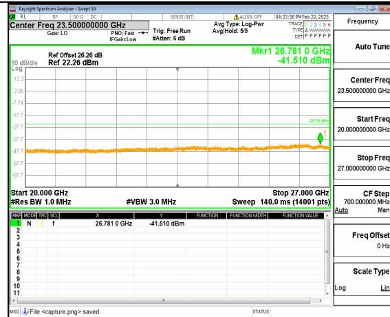
66A_n41 (20GHz-27GHz) 80M DFT-s-OFDM QPSK Inner_1RB_Right Low
