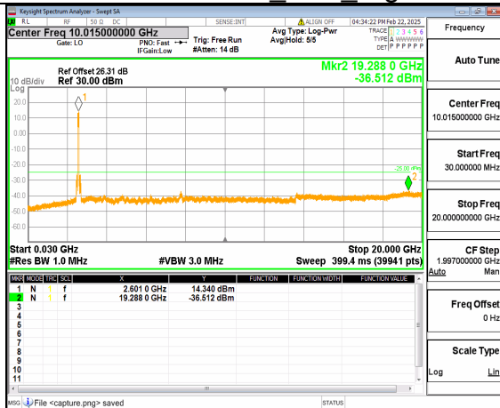
66A_n41 (30MHz-20GHz) 80M DFT-s-OFDM QPSK Outer_Full Mid
