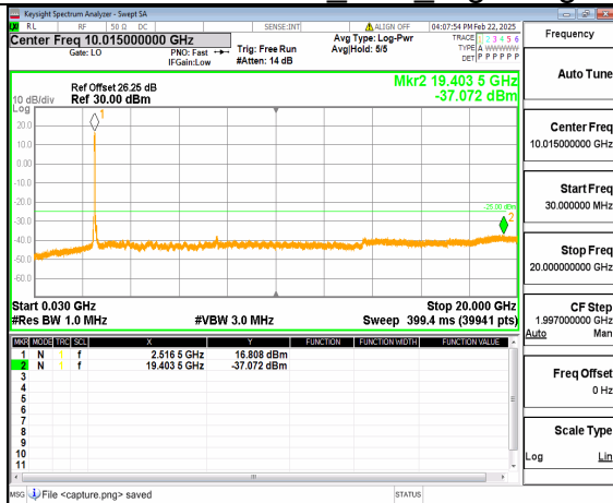
66A_n41 (30MHz-20GHz) 50M DFT-s-OFDM QPSK Outer_Full Low
