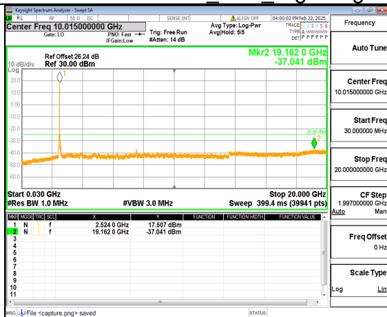
66A_n41 (30MHz-20GHz) 40M DFT-s-OFDM QPSK Outer_Full Low
