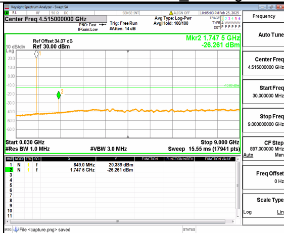
66A_n5 (30MHz-9GHz) 15M DFT-s-OFDM QPSK Inner 1RB Right High
