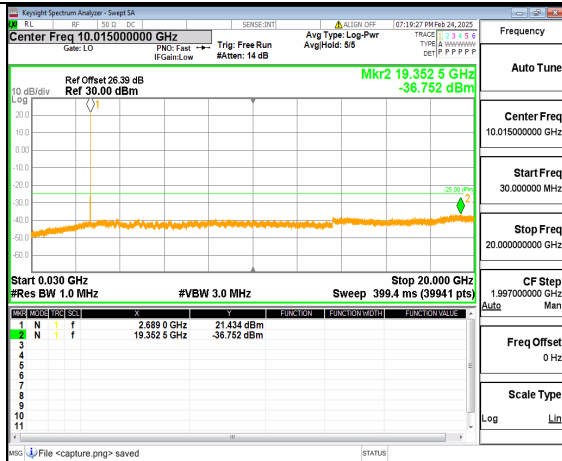
66A_n41 (30MHz-20GHz) 20M DFT-s-OFDM QPSK Inner 1RB Right High
