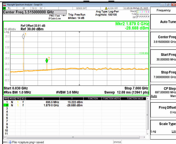
2A_n71 (30MHz-7GHz) 5M DFT-s-OFDM QPSK Outer_Full High
