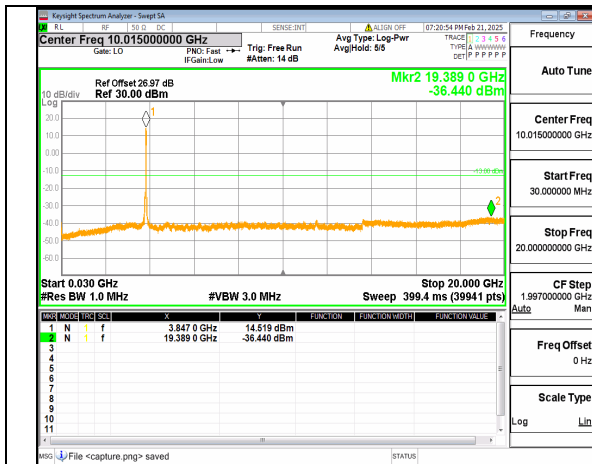
12A_n77(3700-3980MHz) (30MHz-20GHz) 50M DFT-s-OFDM QPSK Outer_Full_Mid
