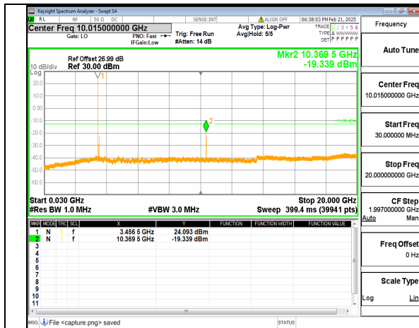
12A_n77(3450-3550MHz) (30MHz-20GHz) 90M DFT-s-OFDM QPSK Inner_1RB_Left Mid
