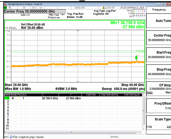
12A_n77(3700-3980MHz) (20GHz-40GHz) 60M DFT-s-OFDM QPSK Inner_1RB_Left Low
