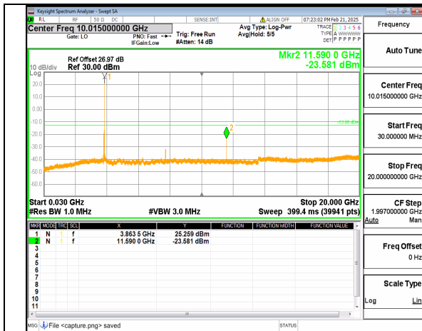
12A_n77(3700-3980MHz) (30MHz-20GHz) 50M DFT-s-OFDM QPSK Inner_1RB_Right Mid
