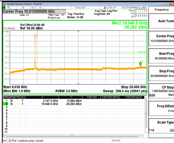
12A_n77(3700-3980MHz) (30MHz-20GHz) 60M DFT-s-OFDM QPSK Outer_Full Low
