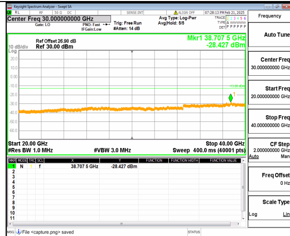
12A_n77(3700-3980MHz) (20GHz-40GHz) 60M DFT-s-OFDM QPSK Outer_Full Low
