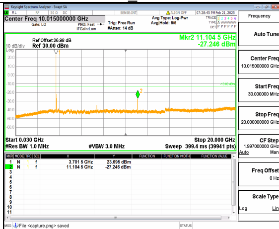
12A_n77(3700-3980MHz) (30MHz-20GHz) 60M DFT-s-OFDM QPSK Inner_1RB_Left Low
