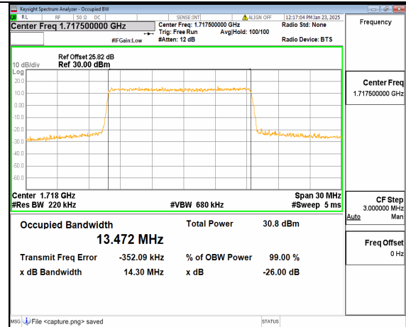
12A_n66 15M DFT-s-OFDM QPSK Outer_Full Low
