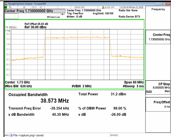
12A_n66 40M DFT-s-OFDM QPSK Outer_Full Low
