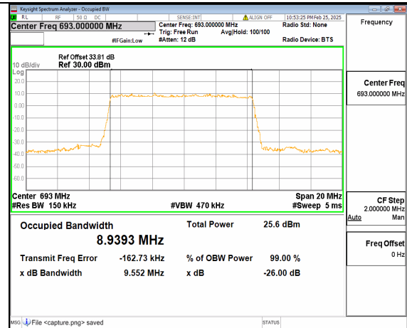
2A_n71 10M DFT-s-OFDM 64QAM Outer_Full High
