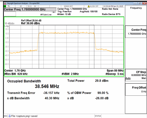
12A_n66 40M DFT-s-OFDM 64QAM Outer_Full High
