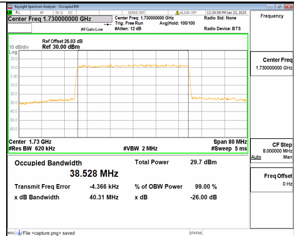
12A_n66 40M DFT-s-OFDM 64QAM Outer_Full Low
