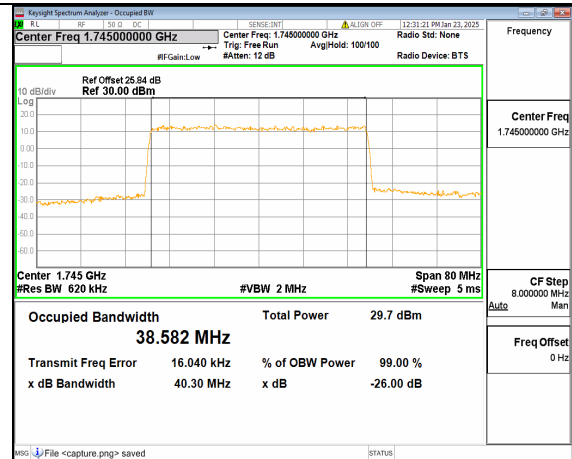
12A_n66 40M DFT-s-OFDM 64QAM Outer_Full Mid
