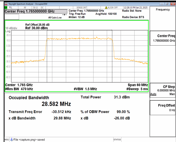
12A_n66 30M DFT-s-OFDM QPSK Outer_Full High
