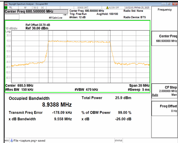
2A_n71 10M DFT-s-OFDM 64QAM Outer_Full Mid
