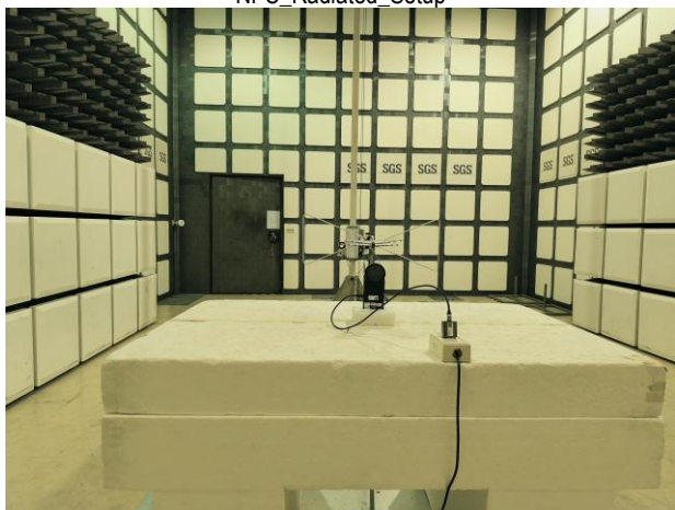
NFC_Radiated_Setup
