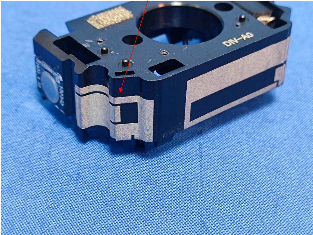
WLAN/Bluetooth Antenna
