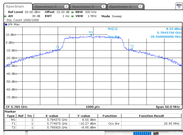
a_5785MHz_Chain 0
