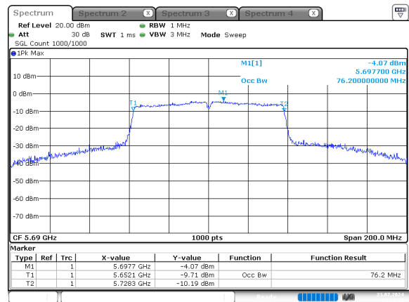
ac80_5690MHz_Chain 0
