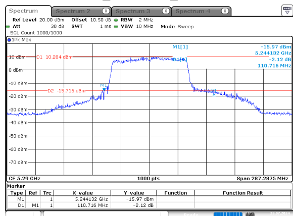
ac80 5290MHz Chain 0
