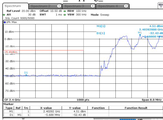
GFSK_Hopping_Lower
