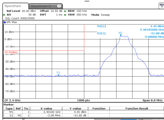
GFSK_Low
