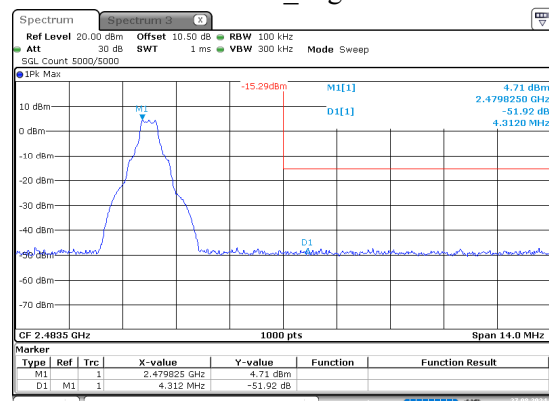
GFSK_High
