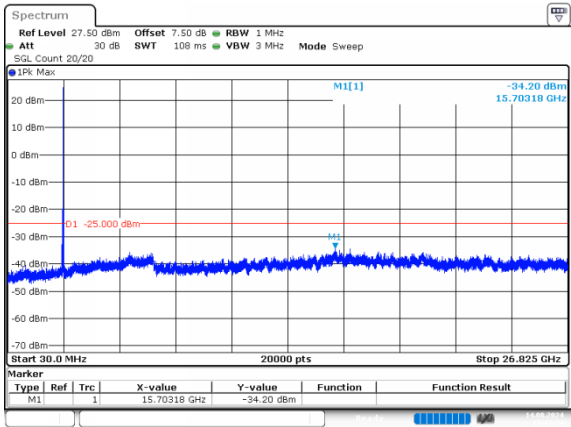
15MHz_High_QPSK_1@0
