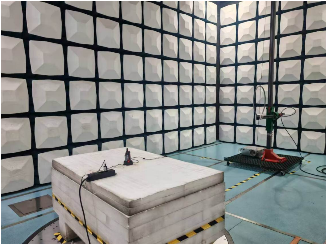
Radiated Emission 9k-30MHz Perpendicular View-Charging base
