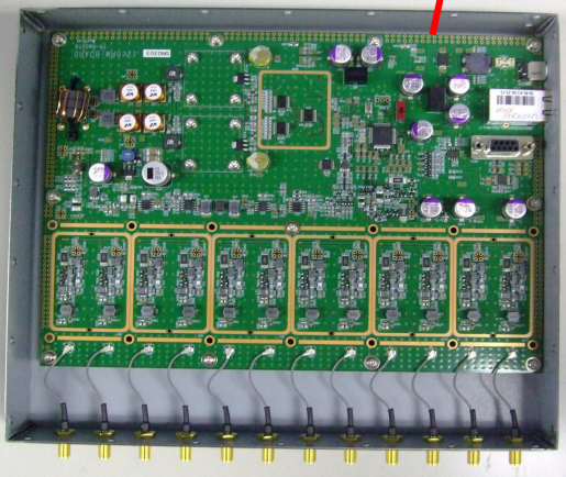
Internal photos RW 12chRW Board
