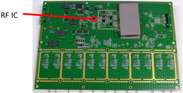
12chRW Board Bottom
