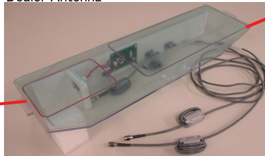
Dealer Antenna
