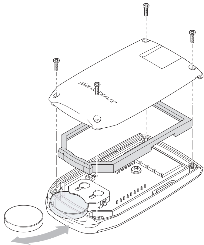
Figure 3-6. Key fob battery replacement.
