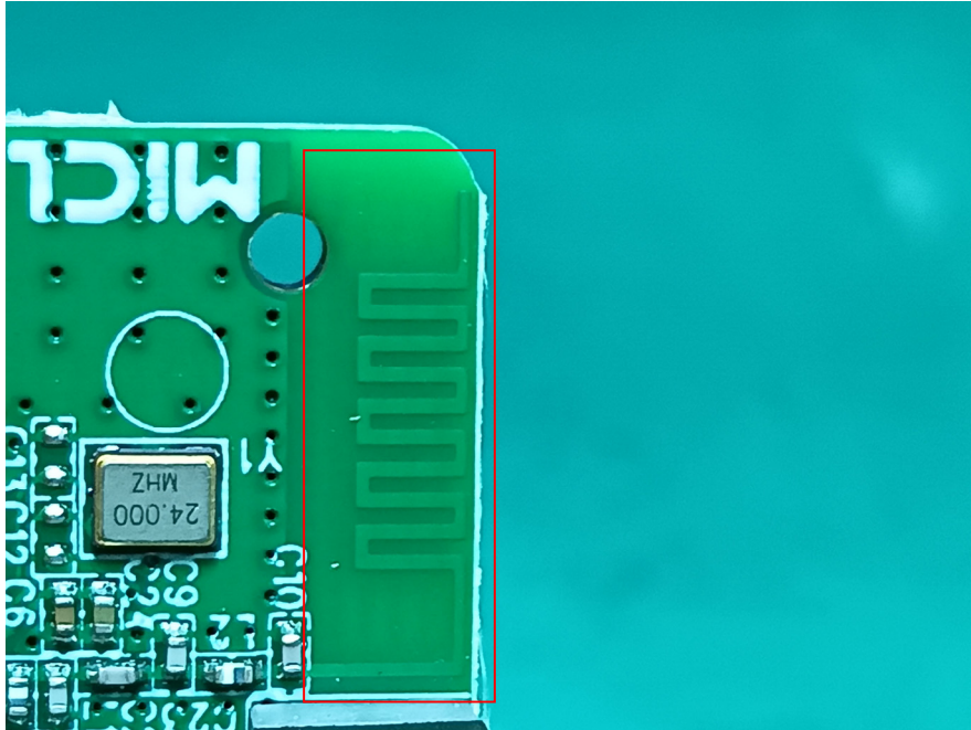
BLE/2.4G Antenna
