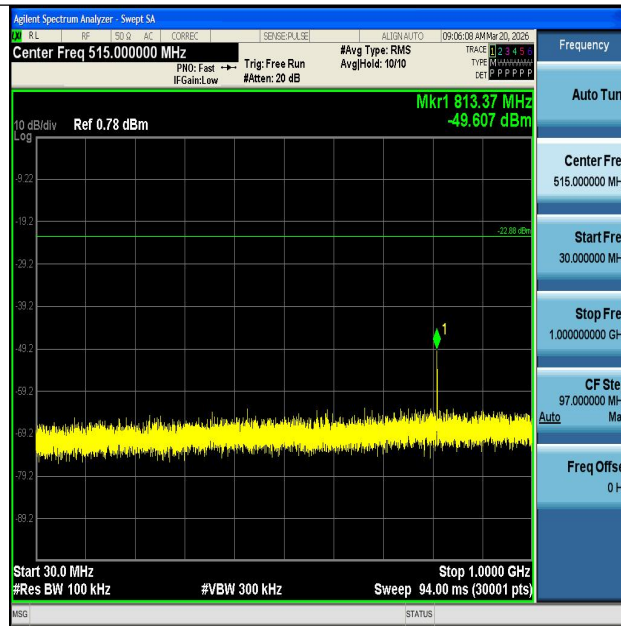
SRD-Ant1-2440-30~1000-PASS
