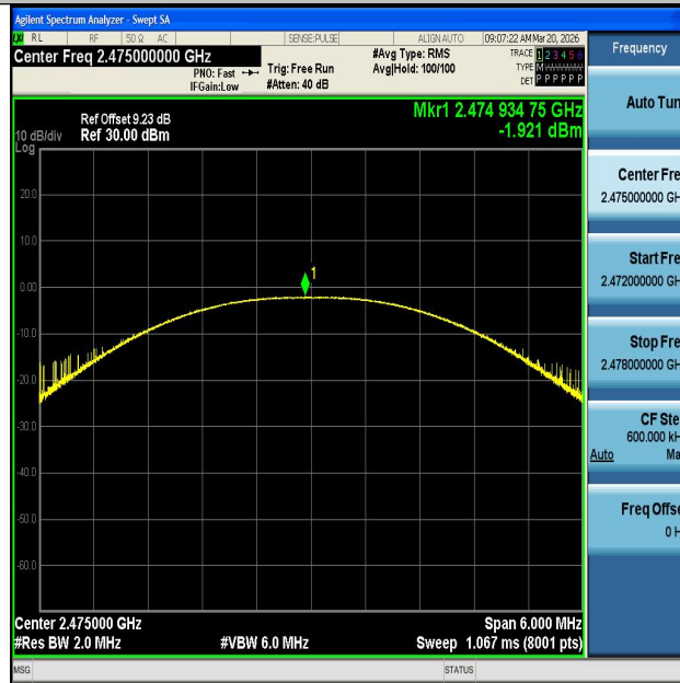
SRD-Ant1-2475-PASS
