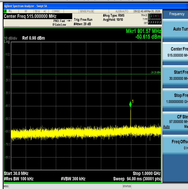
SRD-Ant1-2405-30~1000-PASS
