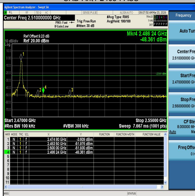
SRD-Ant1-2475-PASS
