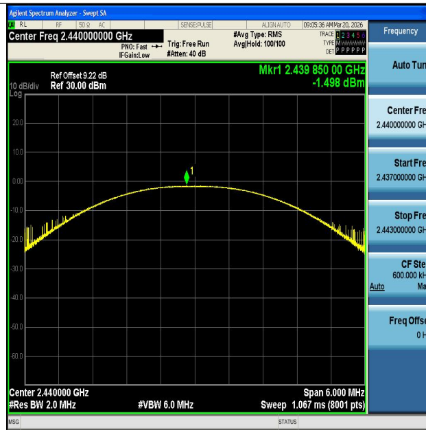
SRD-Ant1-2440-PASS
