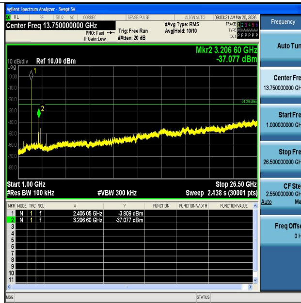
SRD-Ant1-2405-1000~26500-PASS
