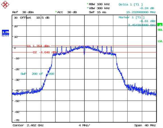
802.11n20_2462MHz 15.232MHz
