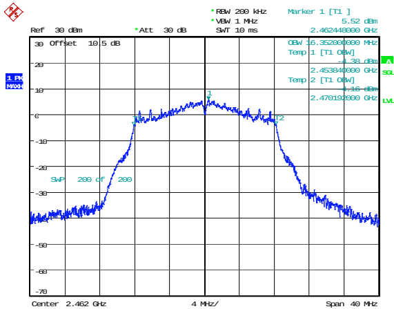
802.11g_2462MHz 16.352MHz
