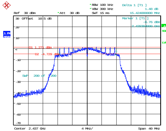
802.11n20_2437MHz 15.424MHz
