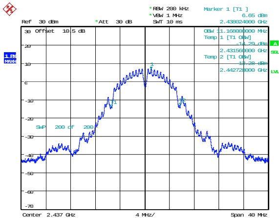
802.11b_2437MHz 11.168MHz
