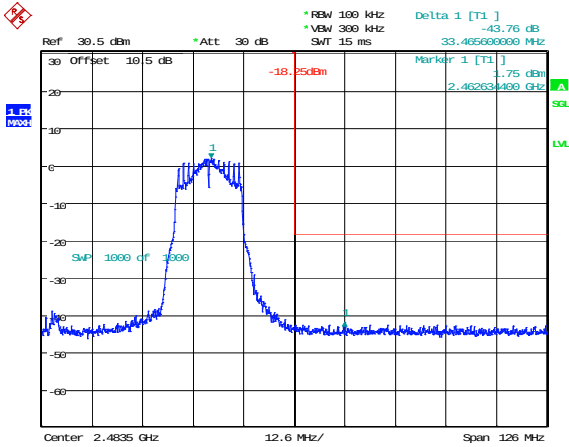
802.11g_2462MHz 43.76dB
