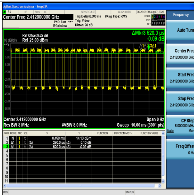
NTNV-11AX20SISO-Ant1-2412
