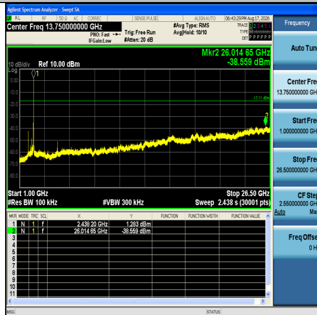
11AX20SISO-Ant1-2437-1000~26500-PASS
