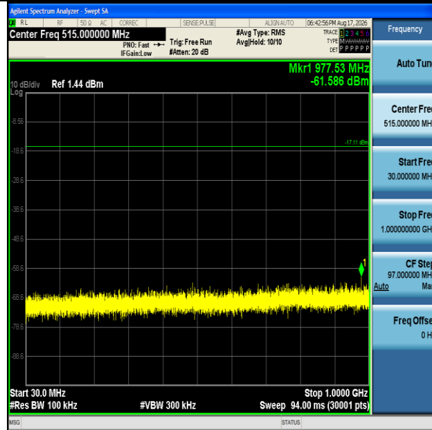
11AX20SISO-Ant1-2437-30~1000-PASS
