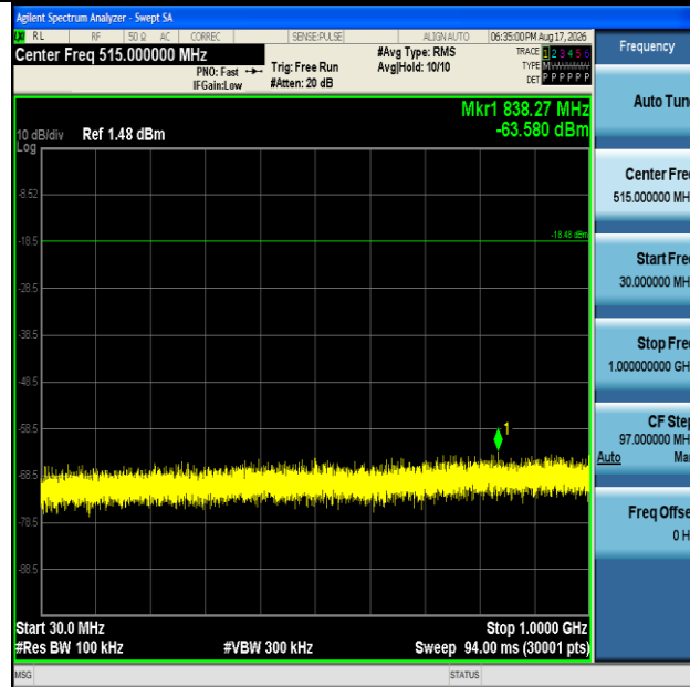
11AX20SISO-Ant1-2412-30~1000-PASS
