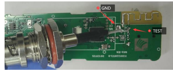
Figure 3: Connection method
