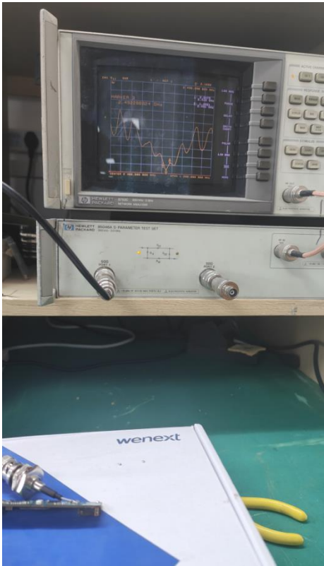
Figure 3: Connection method
