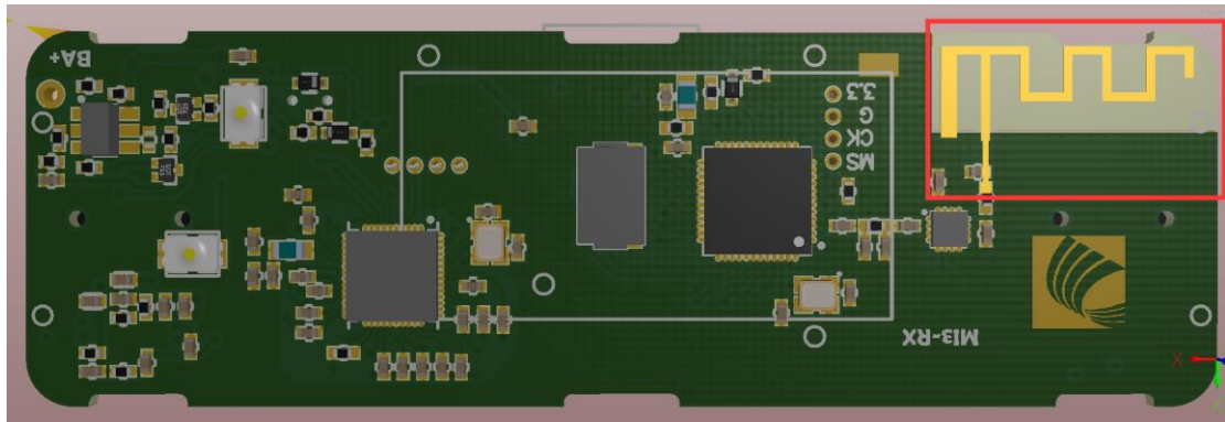
Figure 2: 3D PCB
