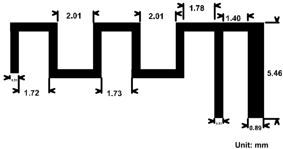
Figure 1: Antenna Dimensions
